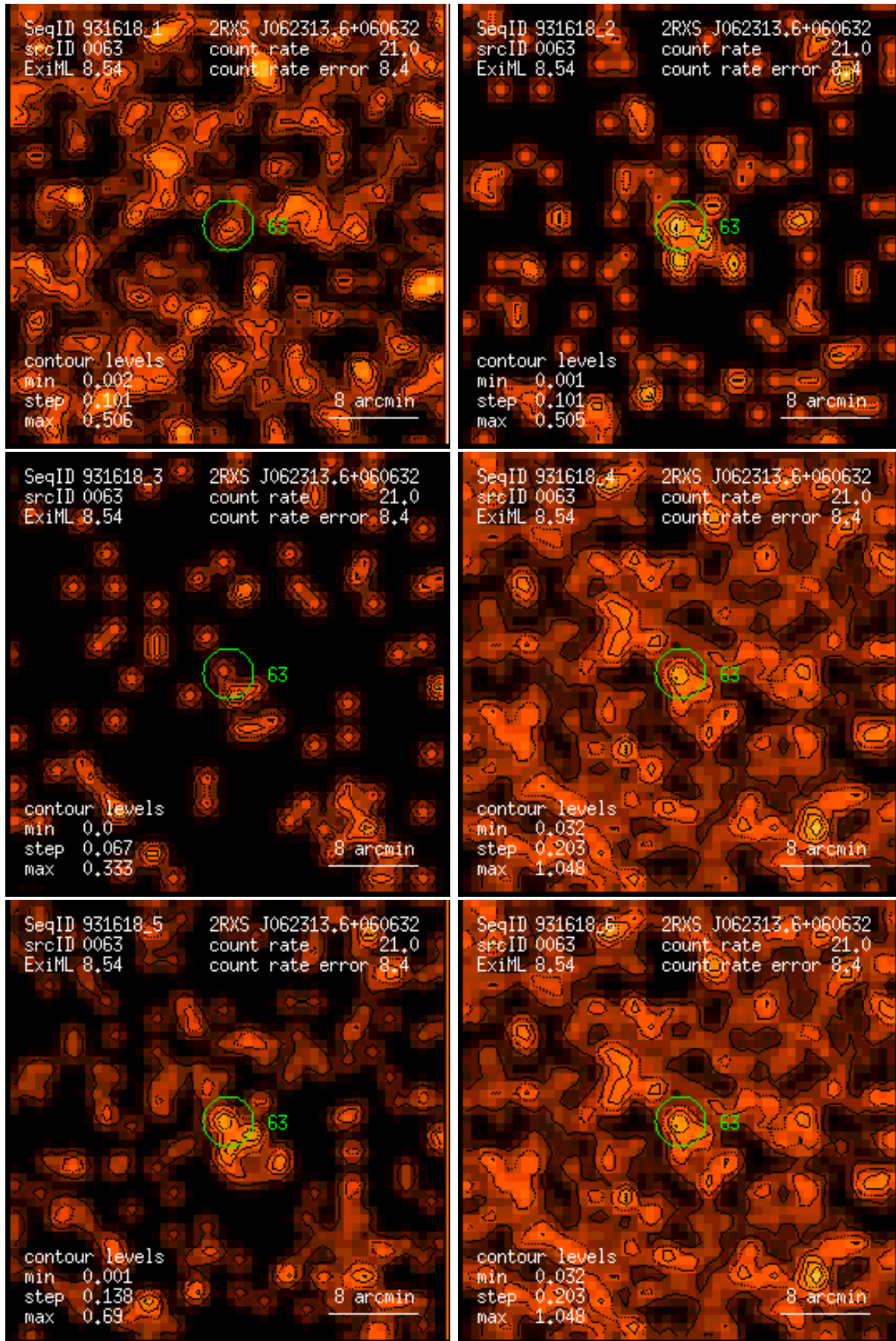
Figure 63: RASS 931618: detection 0063: band rate images, Gaussian filter: (1) PSPC channels 11 – 41, (2) 52 – 90, (3) 91 – 201, (4) 11 – 235, (5) 52 – 201, (6) 11 – 201. Broad band rates in counts/ks. Band rate contour levels in counts/ks/arcmin 2 .
