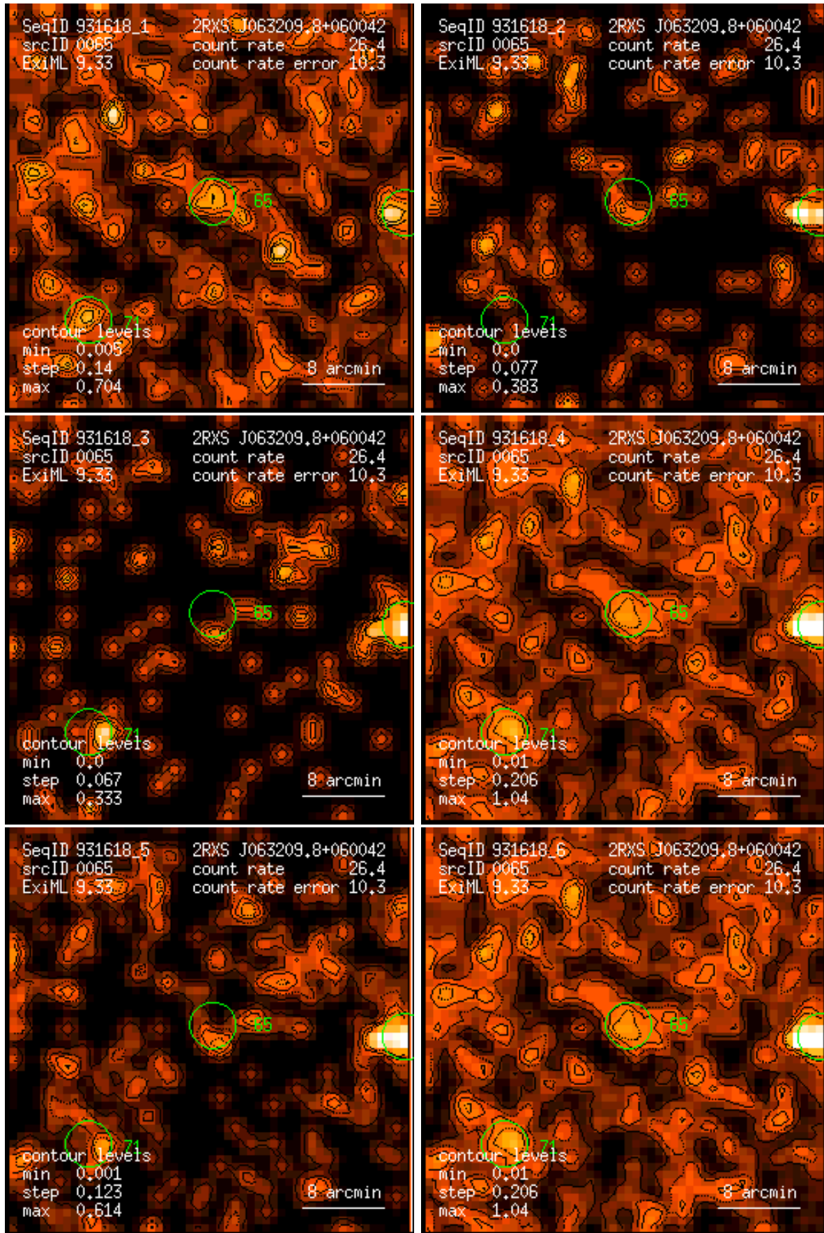
Figure 65: RASS 931618: detection 0065: band rate images, Gaussian filter: (1) PSPC channels 11 – 41, (2) 52 – 90, (3) 91 – 201, (4) 11 – 235, (5) 52 – 201, (6) 11 – 201. Broad band rates in counts/ks. Band rate contour levels in counts/ks/arcmin 2 .
