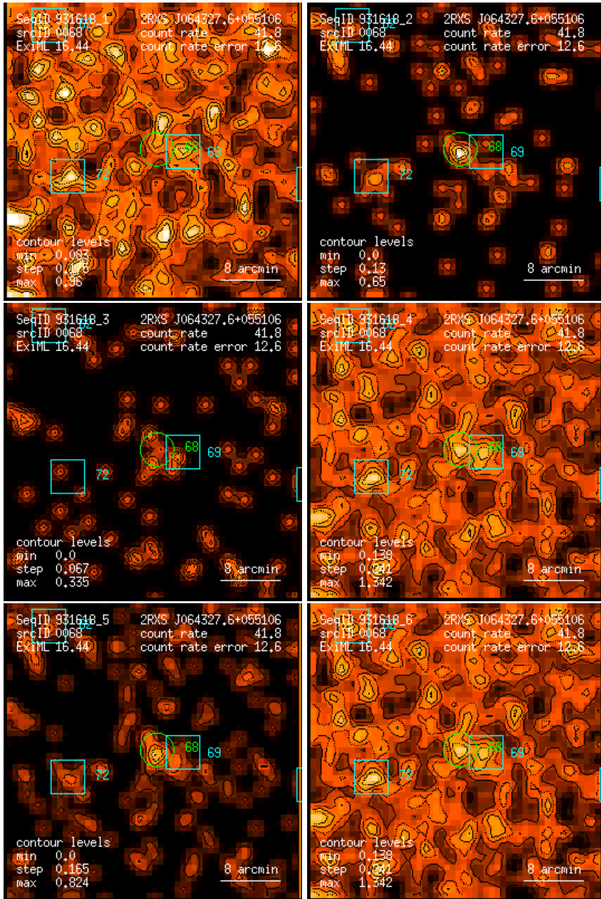
Figure 68: RASS 931618: detection 0068: band rate images, Gaussian filter: (1) PSPC channels 11 – 41, (2) 52 – 90, (3) 91 – 201, (4) 11 – 235, (5) 52 – 201, (6) 11 – 201. Broad band rates in counts/ks. Band rate contour levels in counts/ks/arcmin 2 .
