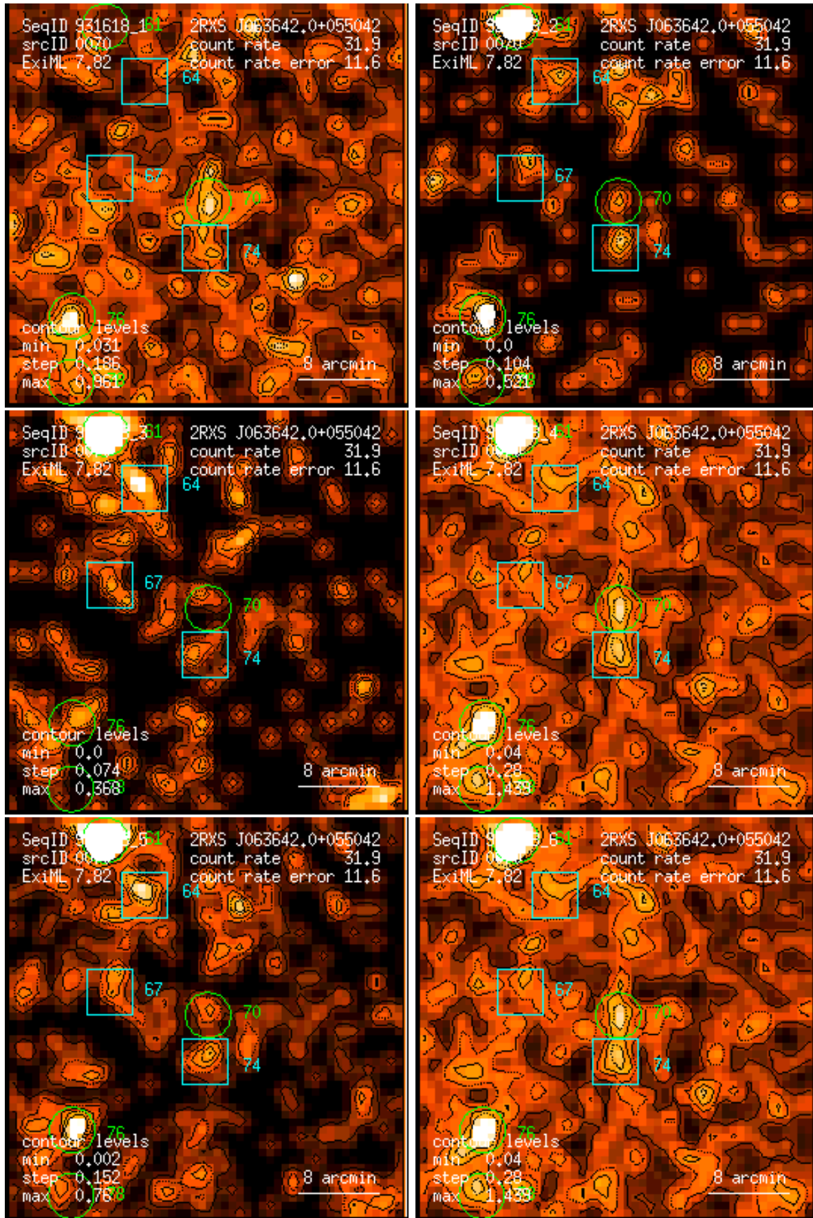
Figure 70: RASS 931618: detection 0070: band rate images, Gaussian filter: (1) PSPC channels 11 – 41, (2) 52 – 90, (3) 91 – 201, (4) 11 – 235, (5) 52 – 201, (6) 11 – 201. Broad band rates in counts/ks. Band rate contour levels in counts/ks/arcmin 2 .
