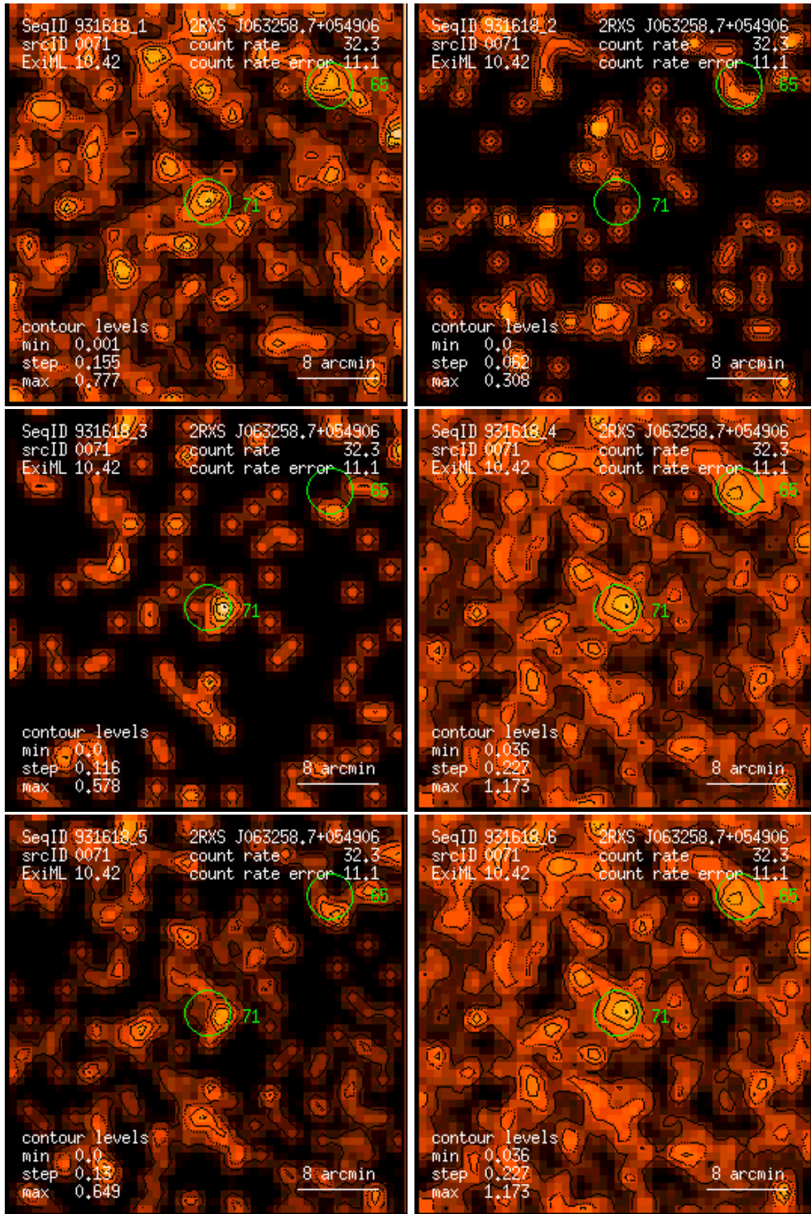
Figure 71: RASS 931618: detection 0071: band rate images, Gaussian filter: (1) PSPC channels 11 – 41, (2) 52 – 90, (3) 91 – 201, (4) 11 – 235, (5) 52 – 201, (6) 11 – 201. Broad band rates in counts/ks. Band rate contour levels in counts/ks/arcmin 2 .
