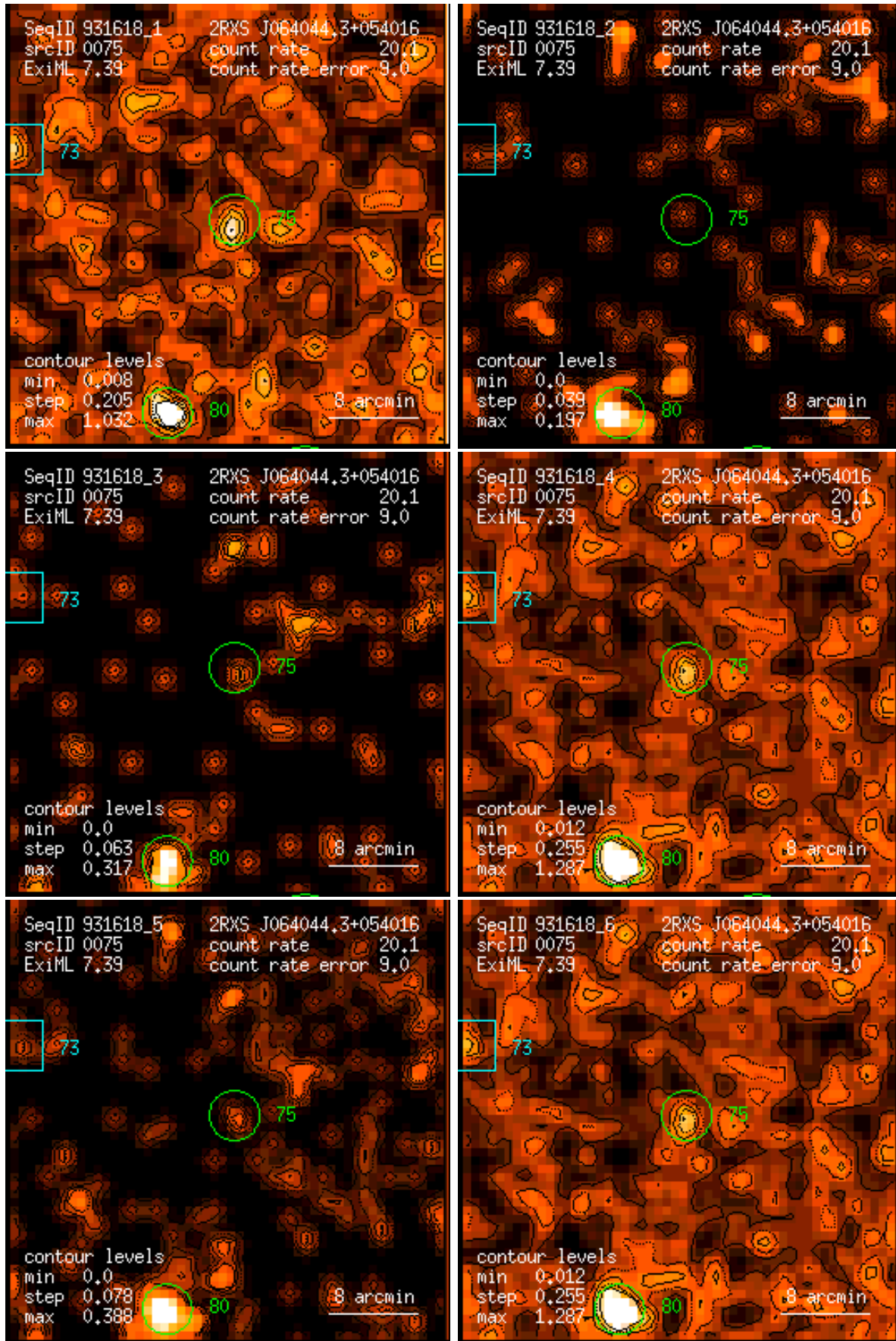
Figure 75: RASS 931618: detection 0075: band rate images, Gaussian filter: (1) PSPP channels 11 – 41, (2) 52 – 90, (3) 91 – 201, (4) 11 – 235, (5) 52 – 201, (6) 11 – 201. Broad band rates in counts/ks. Band rate contour levels in counts/ks/arcmin 2 .
