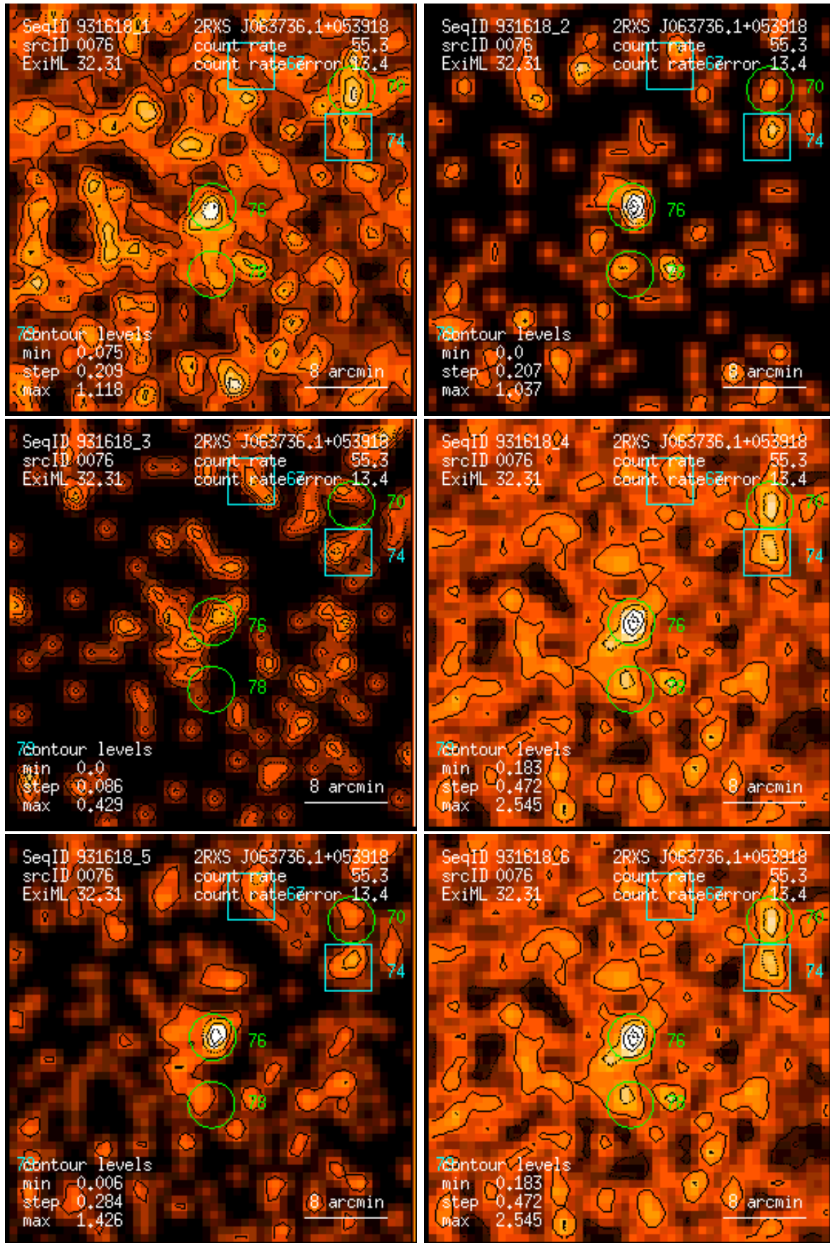
Figure 76: RASS 931618: detection 0076: band rate images, Gaussian filter: (1) PSPC channels 11 – 41, (2) 52 – 90, (3) 91 – 201, (4) 11 – 235, (5) 52 – 201, (6) 11 – 201. Broad band rates in counts/ks. Band rate contour levels in counts/ks/arcmin 2 .
