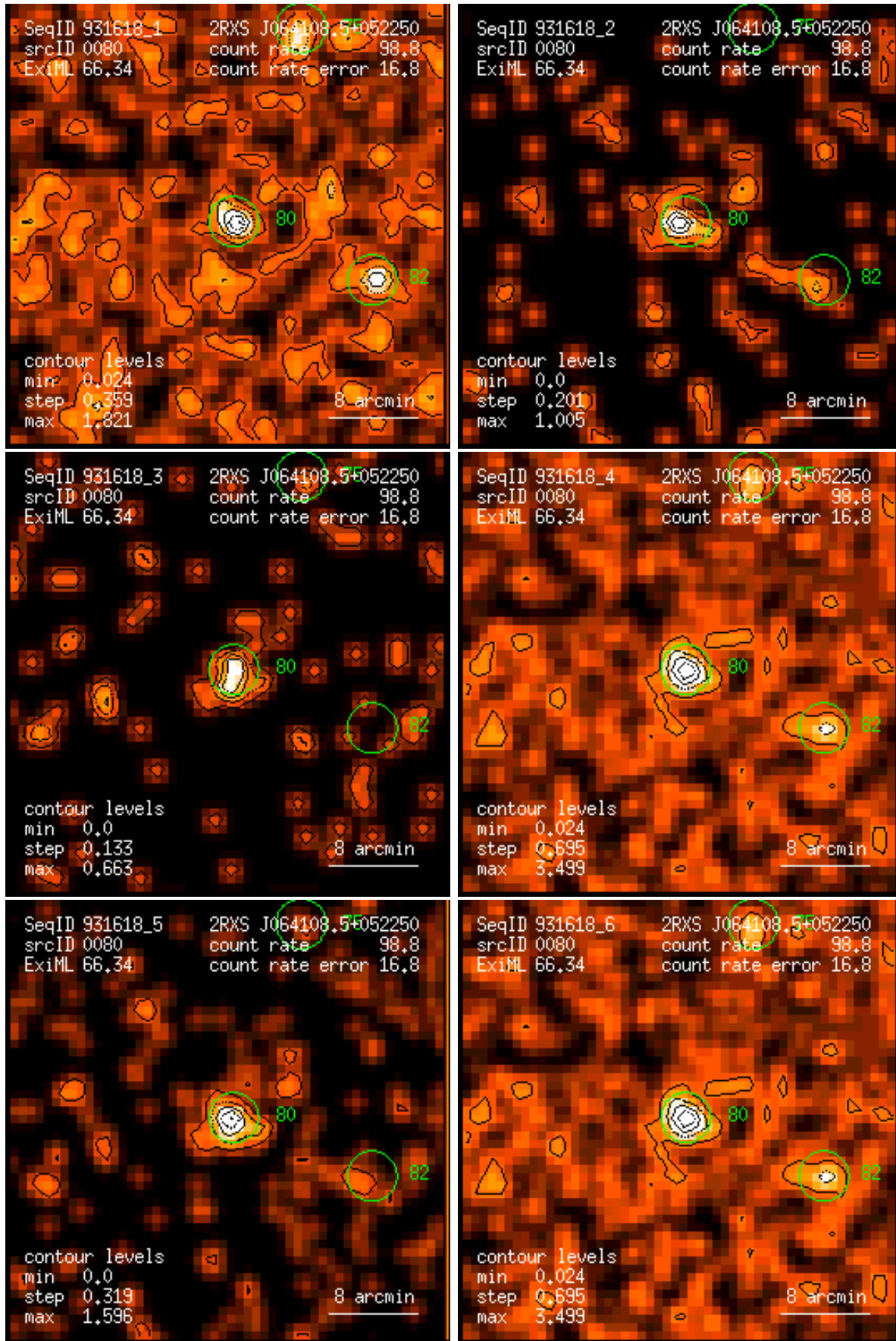
Figure 80: RASS 931618: detection 0080: band rate images, Gaussian filter: (1) PSPC channels 11 – 41, (2) 52 – 90, (3) 91 – 201, (4) 11 – 235, (5) 52 – 201, (6) 11 – 201. Broad band rates in counts/ks. Band rate contour levels in counts/ks/arcmin 2 .
