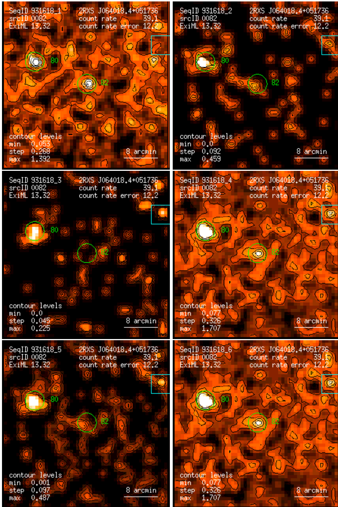
Figure 82: RASS 931618: detection 0082: band rate images, Gaussian filter: (1) PSPC channels 11 – 41, (2) 52 – 90, (3) 91 – 201, (4) 11 – 235, (5) 52 – 201, (6) 11 – 201. Broad band rates in counts/ks. Band rate contour levels in counts/ks/arcmin 2 .
