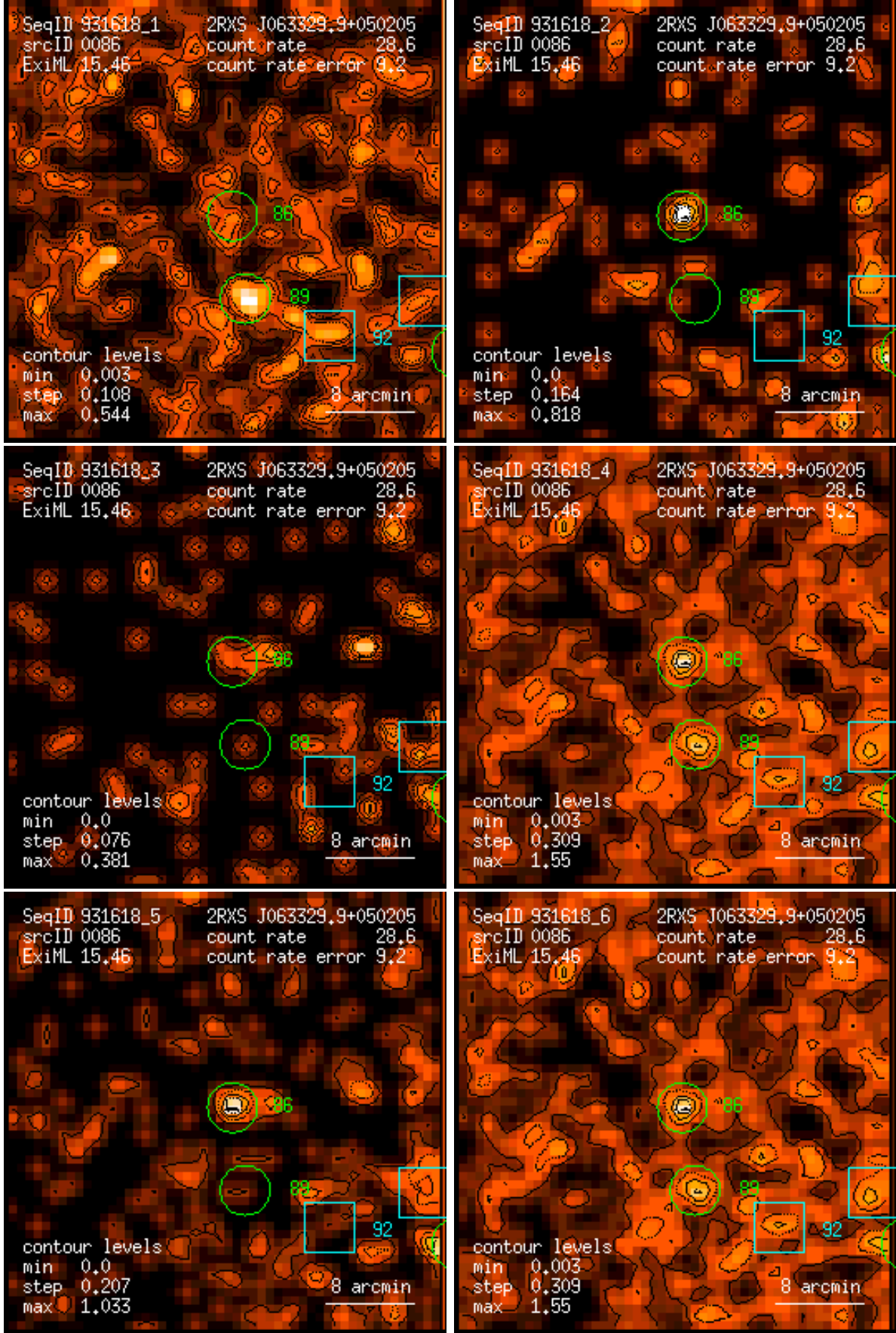
Figure 86: RASS 931618: detection 0086: band rate images, Gaussian filter: (1) PSPC channels 11 – 41, (2) 52 – 90, (3) 91 – 201, (4) 11 – 235, (5) 52 – 201, (6) 11 – 201. Broad band rates in counts/ks. Band rate contour levels in counts/ks/arcmin 2 .
