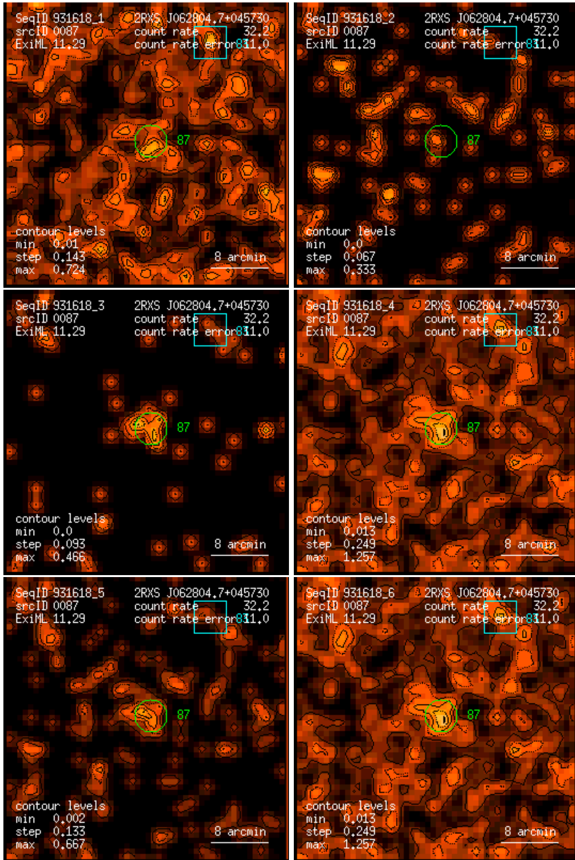
Figure 87: RASS 931618: detection 0087: band rate images, Gaussian filter: (1) PSPC channels 11 – 41, (2) 52 – 90, (3) 91 – 201, (4) 11 – 235, (5) 52 – 201, (6) 11 – 201. Broad band rates in counts/ks. Band rate contour levels in counts/ks/arcmin 2 .
