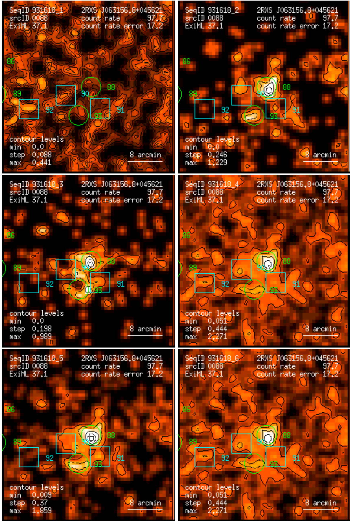
Figure 88: RASS 931618: detection 0088: band rate images, Gaussian filter: (1) PSPC channels 11 – 41, (2) 52 – 90, (3) 91 – 201, (4) 11 – 235, (5) 52 – 201, (6) 11 – 201. Broad band rates in counts/ks. Band rate contour levels in counts/ks/arcmin 2 .
