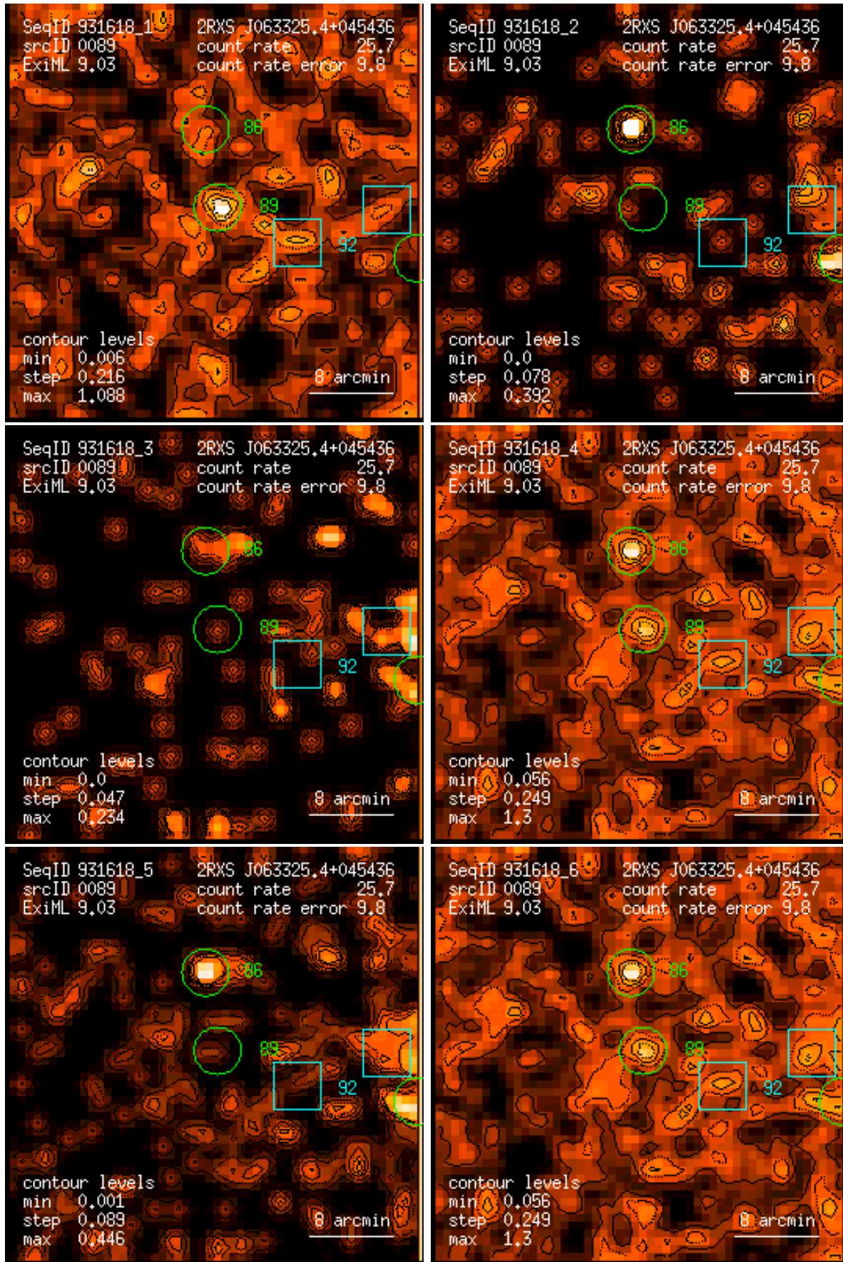
Figure 89: RASS 931618: detection 0089: band rate images, Gaussian filter: (1) PSPC channels 11 – 41, (2) 52 – 90, (3) 91 – 201, (4) 11 – 235, (5) 52 – 201, (6) 11 – 201. Broad band rates in counts/ks. Band rate contour levels in counts/ks/arcmin 2 .
