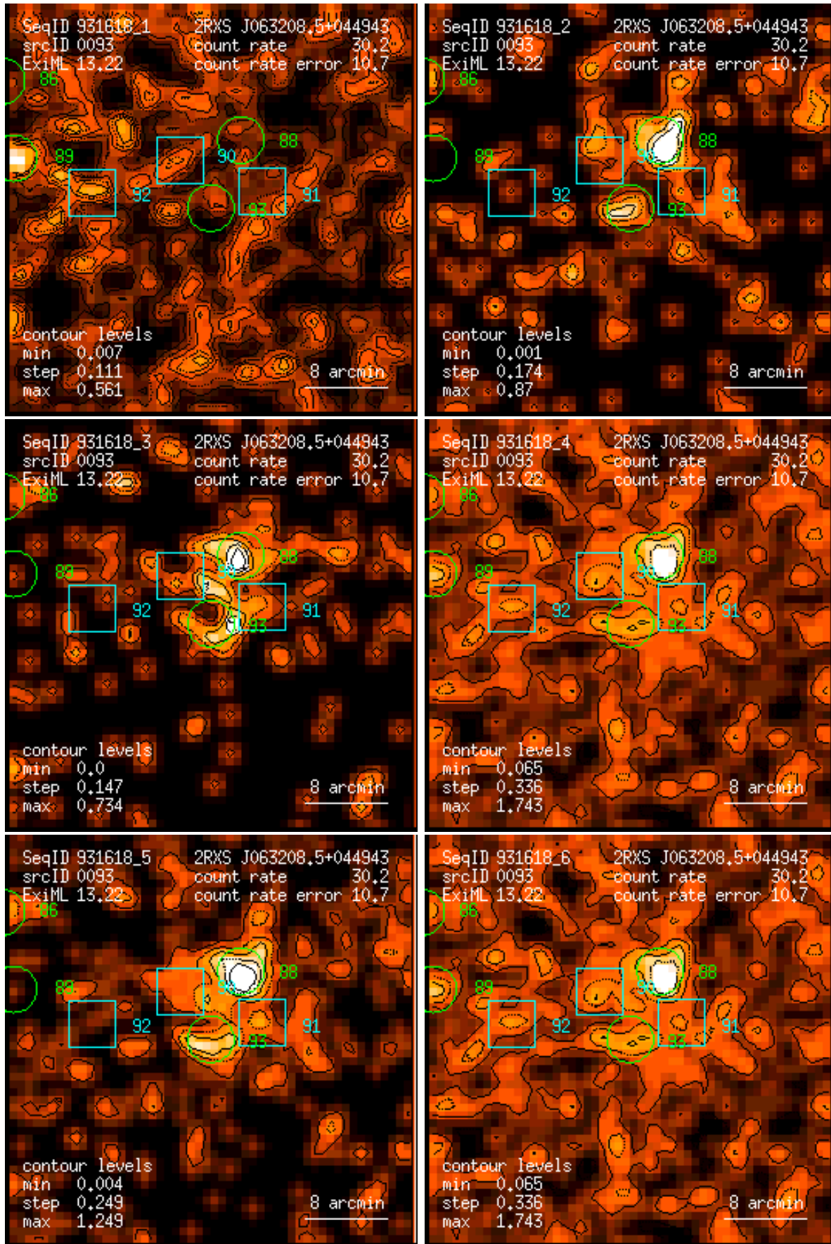
Figure 93: RASS 931618: detection 0093: band rate images, Gaussian filter: (1) PSPC channels 11 – 41, (2) 52 – 90, (3) 91 – 201, (4) 11 – 235, (5) 52 – 201, (6) 11 – 201. Broad band rates in counts/ks. Band rate contour levels in counts/ks/arcmin 2 .
