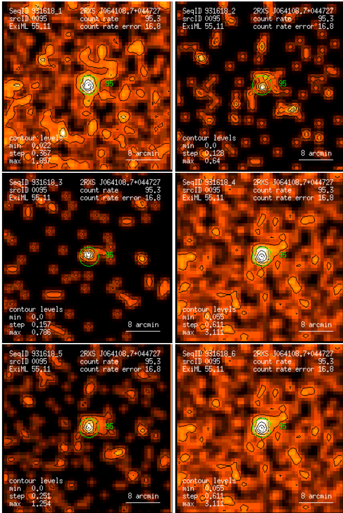
Figure 95: RASS 931618: detection 0095: band rate images, Gaussian filter: (1) PSPC channels 11 – 41, (2) 52 – 90, (3) 91 – 201, (4) 11 – 235, (5) 52 – 201, (6) 11 – 201. Broad band rates in counts/ks. Band rate contour levels in counts/ks/arcmin 2 .
