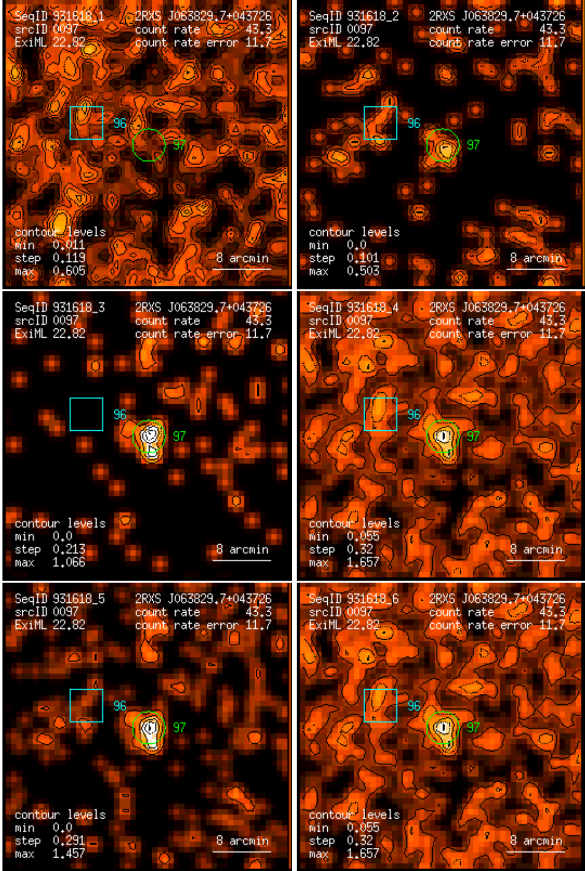
Figure 97: RASS 931618: detection 0097: band rate images, Gaussian filter: (1) PSPC channels 11 – 41, (2) 52 – 90, (3) 91 – 201, (4) 11 – 235, (5) 52 – 201, (6) 11 – 201. Broad band rates in counts/ks. Band rate contour levels in counts/ks/arcmin 2 .
