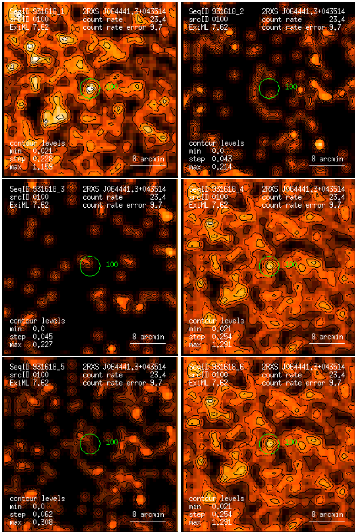
Figure 100: RASS 931618: detection 0100: band rate images, Gaussian filter: (1) PSPC channels 11 – 41, (2) 52 – 90, (3) 91 – 201, (4) 11 – 235, (5) 52 – 201, (6) 11 – 201. Broad band rates in counts/ks. Band rate contour levels in counts/ks/arcmin 2 .
