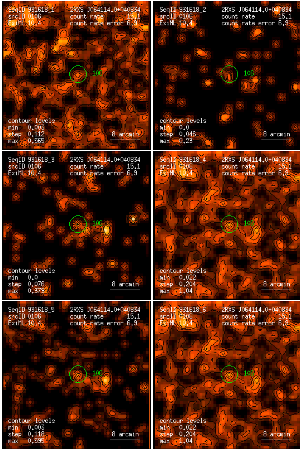
Figure 106: RASS 931618: detection 0106: band rate images, Gaussian filter: (1) PSPC channels 11 – 41, (2) 52 – 90, (3) 91 – 201, (4) 11 – 235, (5) 52 – 201, (6) 11 – 201. Broad band rates in counts/ks. Band rate contour levels in counts/ks/arcmin 2 .
