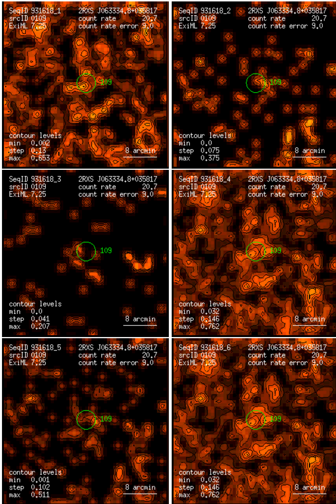
Figure 109: RASS 931618: detection 0109: band rate images, Gaussian filter: (1) PSPC channels 11 – 41, (2) 52 – 90, (3) 91 – 201, (4) 11 – 235, (5) 52 – 201, (6) 11 – 201. Broad band rates in counts/ks. Band rate contour levels in counts/ks/arcmin 2 .
