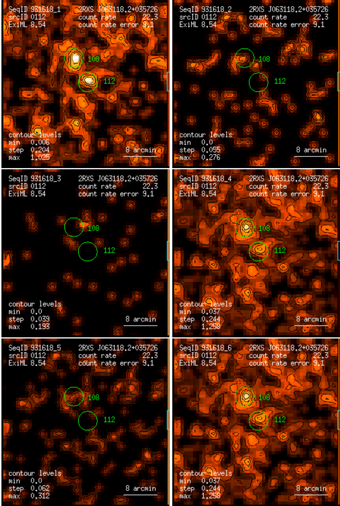
Figure 112: RASS 931618: detection 0112: band rate images, Gaussian filter: (1) PSPC channels 11 – 41, (2) 52 – 90, (3) 91 – 201, (4) 11 – 235, (5) 52 – 201, (6) 11 – 201. Broad band rates in counts/ks. Band rate contour levels in counts/ks/arcmin 2 .
