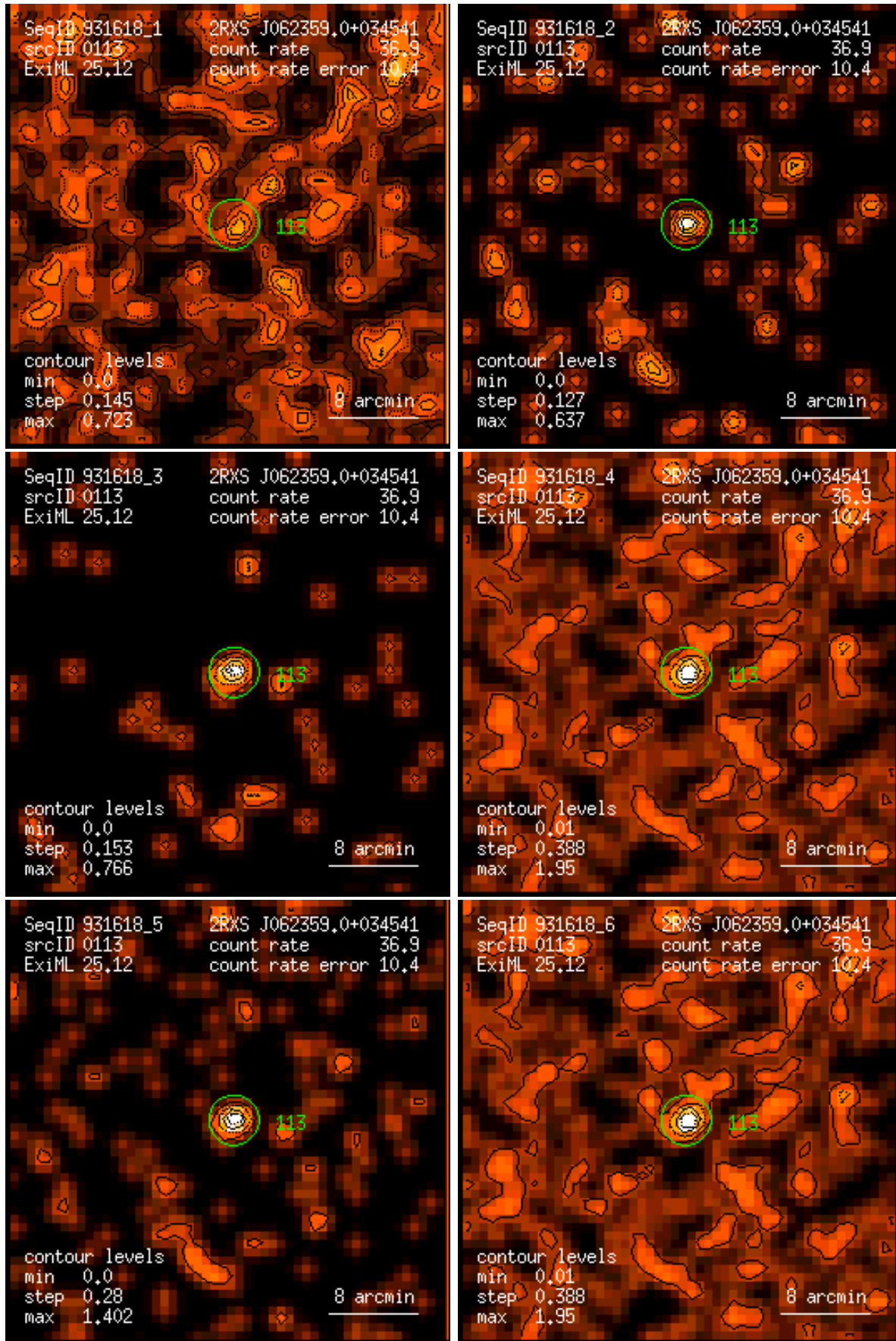
Figure 113: RASS 931618: detection 0113: band rate images, Gaussian filter: (1) PSPC channels 11 – 41, (2) 52 – 90, (3) 91 – 201, (4) 11 – 235, (5) 52 – 201, (6) 11 – 201. Broad band rates in counts/ks. Band rate contour levels in counts/ks/arcmin 2 .
