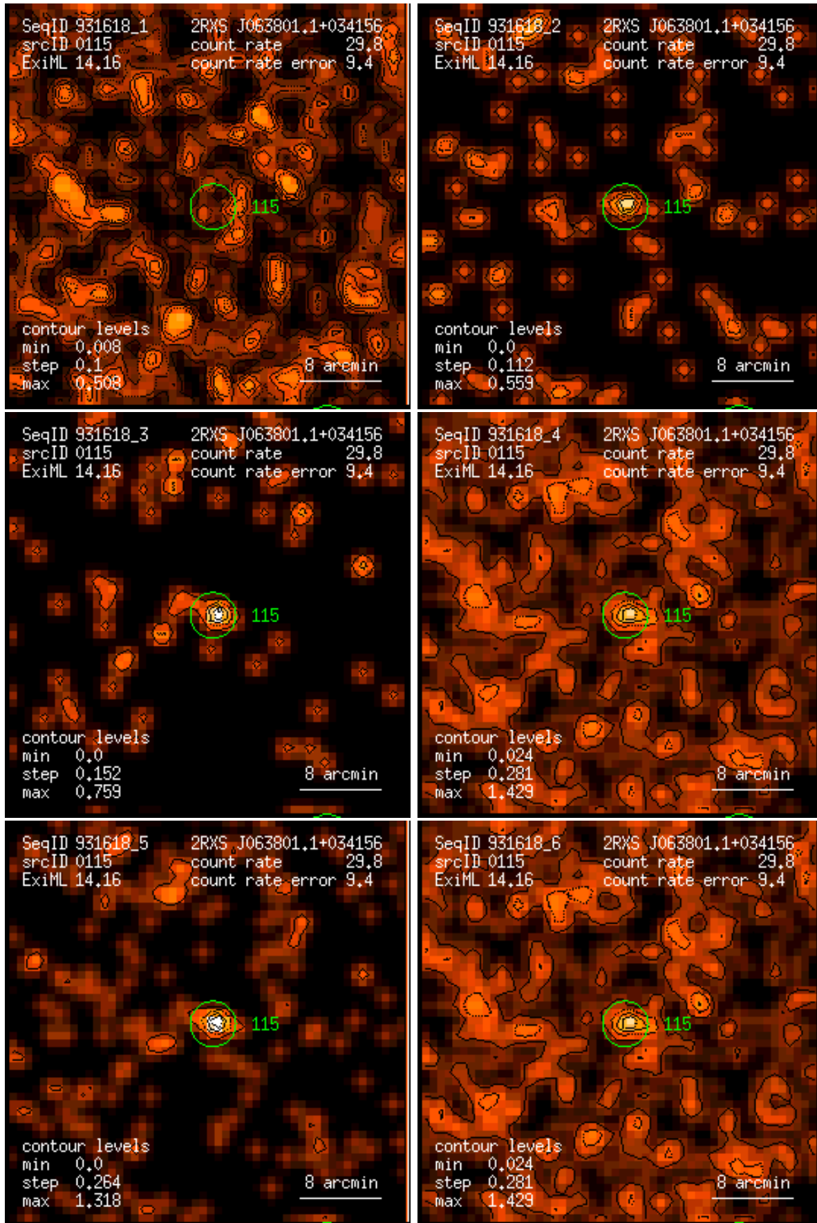
Figure 115: RASS 931618: detection 0115: band rate images, Gaussian filter: (1) PSPC channels 11 – 41, (2) 52 – 90, (3) 91 – 201, (4) 11 – 235, (5) 52 – 201, (6) 11 – 201. Broad band rates in counts/ks. Band rate contour levels in counts/ks/arcmin 2 .
