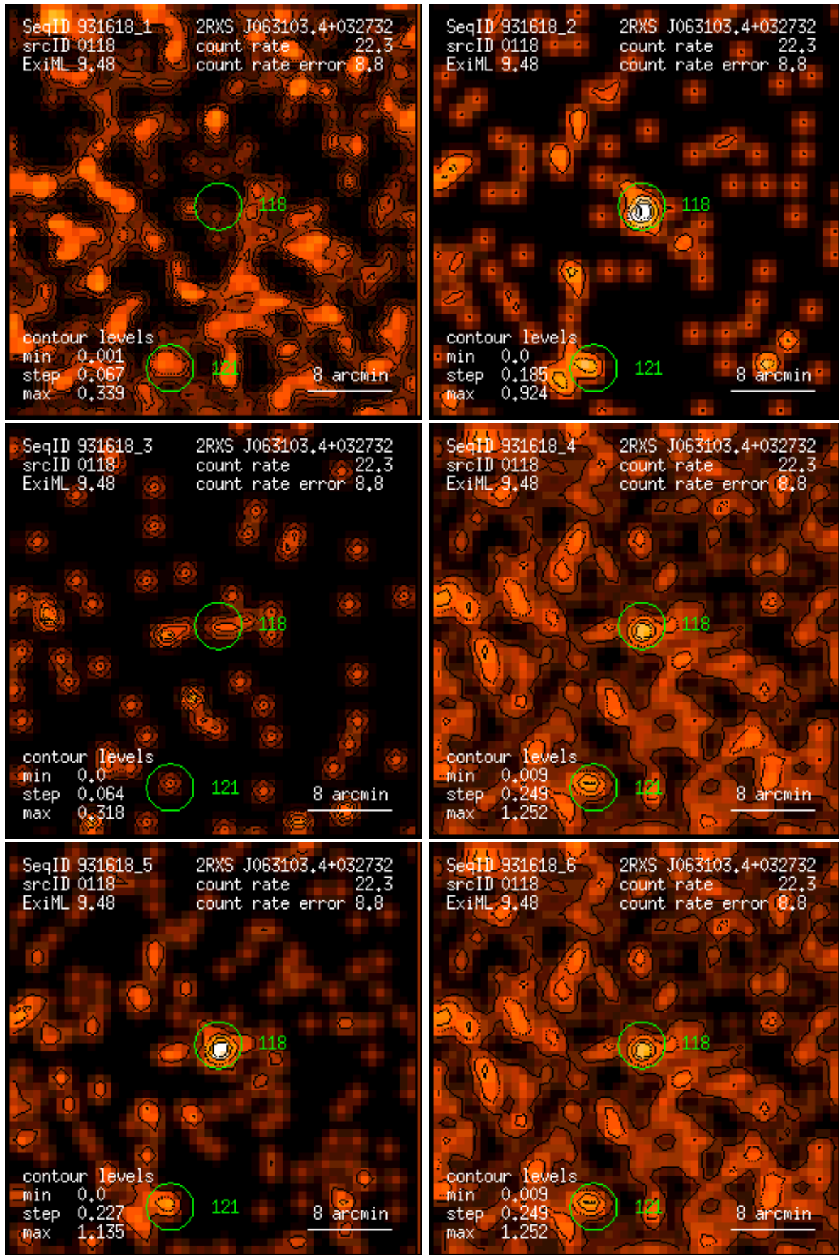
Figure 118: RASS 931618: detection 0118: band rate images, Gaussian filter: (1) PSPC channels 11 – 41, (2) 52 – 90, (3) 91 – 201, (4) 11 – 235, (5) 52 – 201, (6) 11 – 201. Broad band rates in counts/ks. Band rate contour levels in counts/ks/arcmin 2 .
