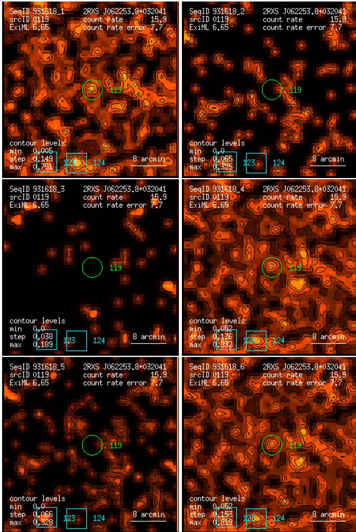
Figure 119: RASS 931618: detection 0119: band rate images, Gaussian filter: (1) PSPC channels 11 – 41, (2) 52 – 90, (3) 91 – 201, (4) 11 – 235, (5) 52 – 201, (6) 11 – 201. Broad band rates in counts/ks. Band rate contour levels in counts/ks/arcmin 2 .
