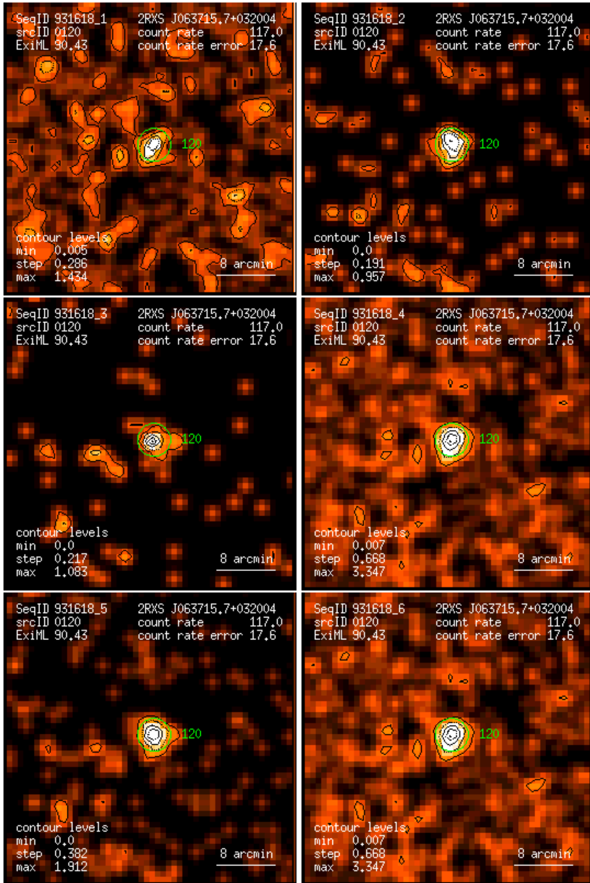
Figure 120: RASS 931618: detection 0120: band rate images, Gaussian filter: (1) PSPC channels 11 – 41, (2) 52 – 90, (3) 91 – 201, (4) 11 – 235, (5) 52 – 201, (6) 11 – 201. Broad band rates in counts/ks. Band rate contour levels in counts/ks/arcmin 2 .
