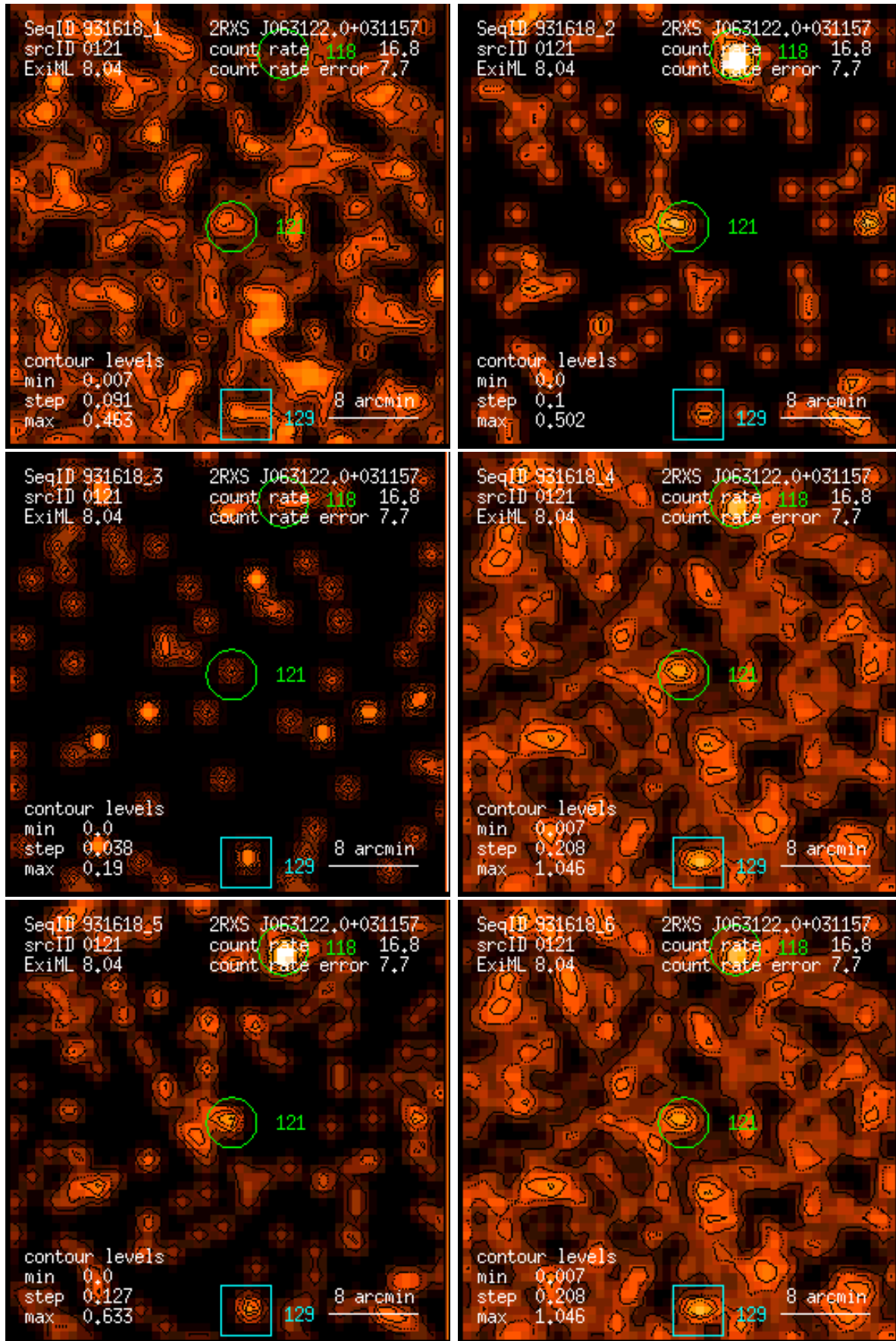
Figure 121: RASS 931618: detection 0121: band rate images, Gaussian filter: (1) PSPC channels 11 – 41, (2) 52 – 90, (3) 91 – 201, (4) 11 – 235, (5) 52 – 201, (6) 11 – 201. Broad band rates in counts/ks. Band rate contour levels in counts/ks/arcmin 2 .
