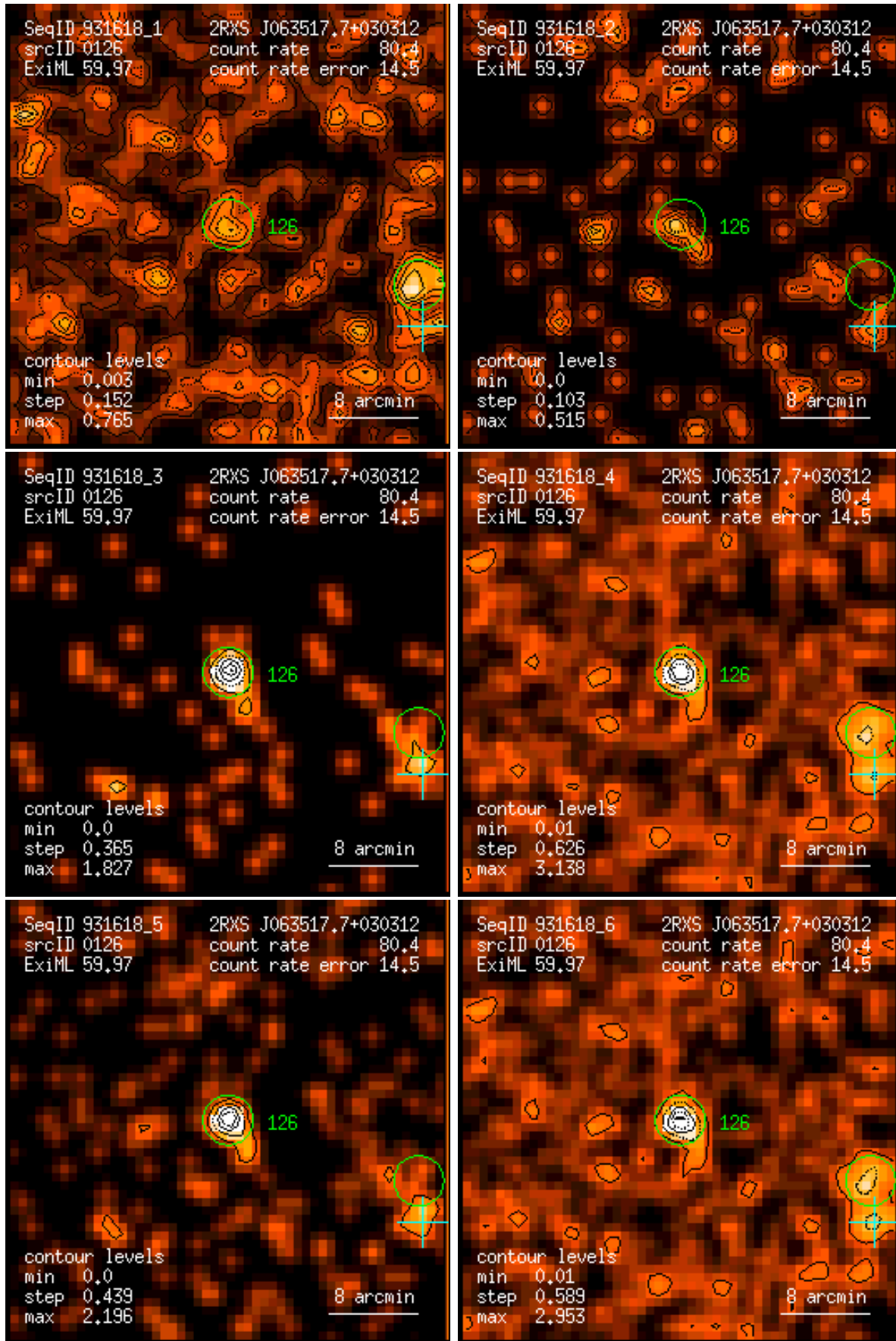
Figure 126: RASS 931618: detection 0126: band rate images, Gaussian filter: (1) PSPC channels 11 – 41, (2) 52 – 90, (3) 91 – 201, (4) 11 – 235, (5) 52 – 201, (6) 11 – 201. Broad band rates in counts/ks. Band rate contour levels in counts/ks/arcmin 2 .
