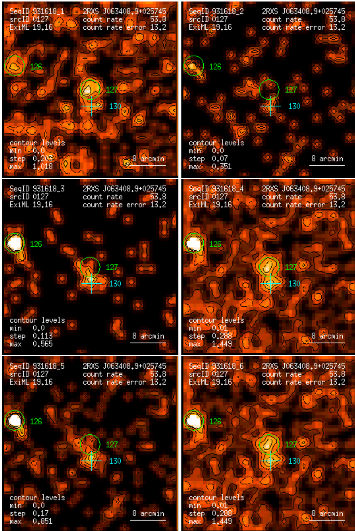
Figure 127: RASS 931618: detection 0127: band rate images, Gaussian filter: (1) PSPC channels 11 – 41, (2) 52 – 90, (3) 91 – 201, (4) 11 – 235, (5) 52 – 201, (6) 11 – 201. Broad band rates in counts/ks. Band rate contour levels in counts/ks/arcmin 2 .
