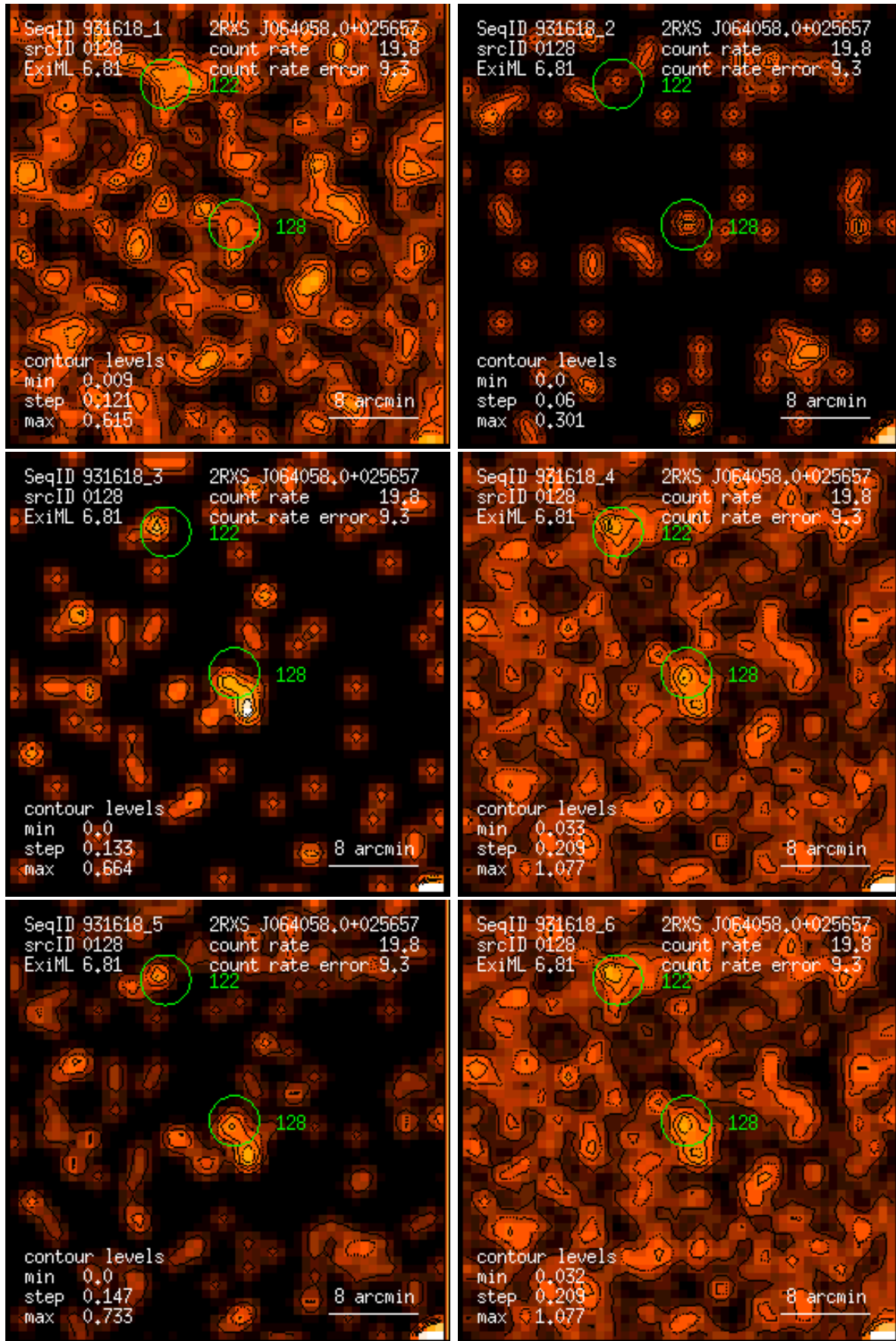
Figure 128: RASS 931618: detection 0128: band rate images, Gaussian filter: (1) PSPC channels 11 – 41, (2) 52 – 90, (3) 91 – 201, (4) 11 – 235, (5) 52 – 201, (6) 11 – 201. Broad band rates in counts/ks. Band rate contour levels in counts/ks/arcmin 2 .
