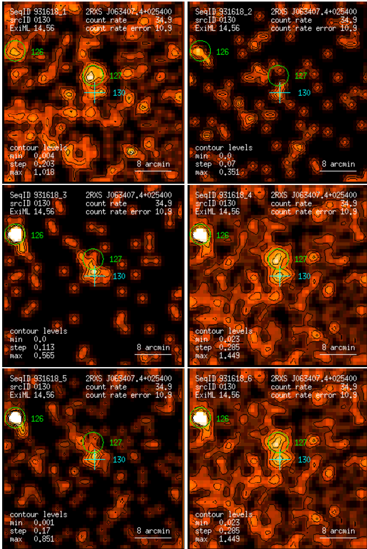
Figure 130: RASS 931618: detection 0130: band rate images, Gaussian filter: (1) PSPC channels 11 – 41, (2) 52 – 90, (3) 91 – 201, (4) 11 – 235, (5) 52 – 201, (6) 11 – 201. Broad band rates in counts/ks. Band rate contour levels in counts/ks/arcmin 2 .
