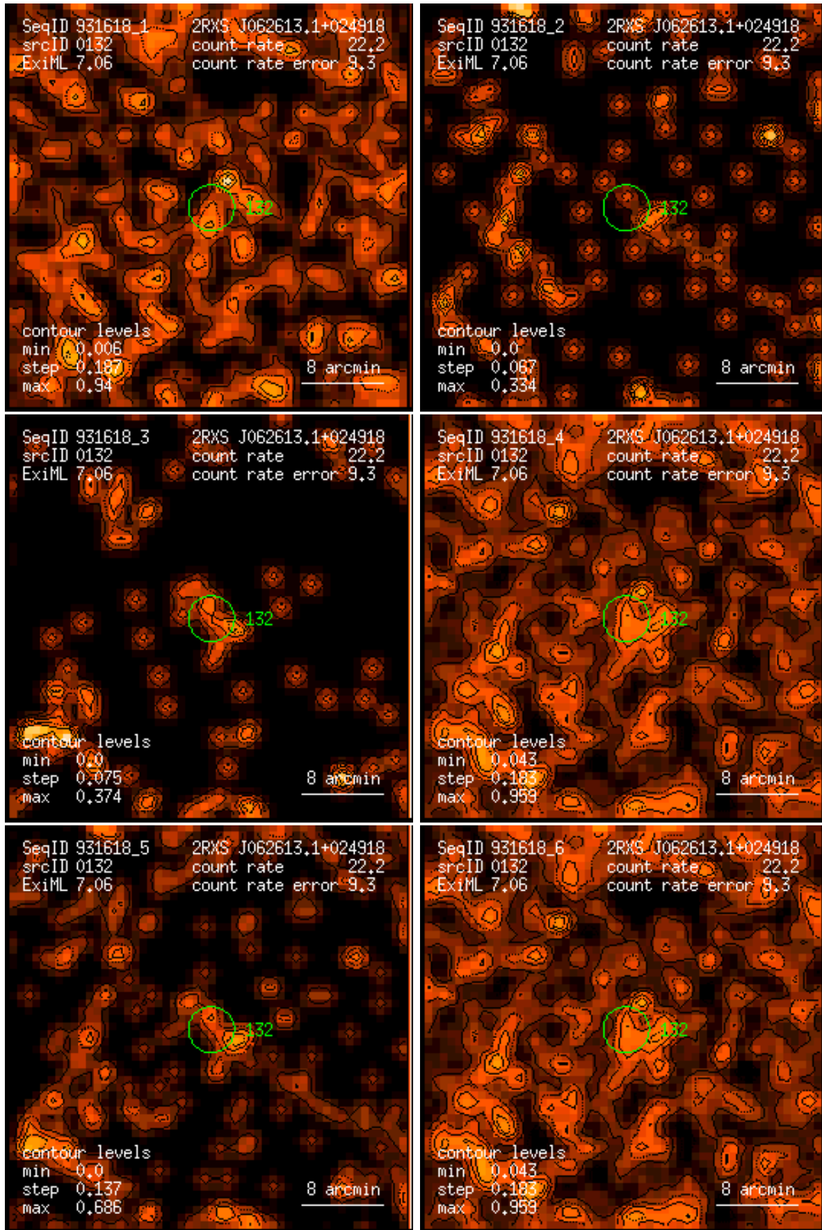
Figure 132: RASS 931618: detection 0132: band rate images, Gaussian filter: (1) PSPC channels 11 – 41, (2) 52 – 90, (3) 91 – 201, (4) 11 – 235, (5) 52 – 201, (6) 11 – 201. Broad band rates in counts/ks. Band rate contour levels in counts/ks/arcmin 2 .
