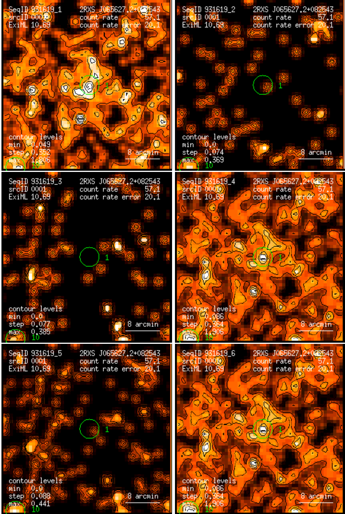
Figure 1: RASS 931619: detection 0001: band rate images, Gaussian filter: (1) PSPC channels 11 – 41, (2) 52 – 90, (3) 91 – 201, (4) 11 – 235, (5) 52 – 201, (6) 11 – 201. Broad band rates in counts/ks. Band rate contour levels in counts/ks/arcmin 2 .
