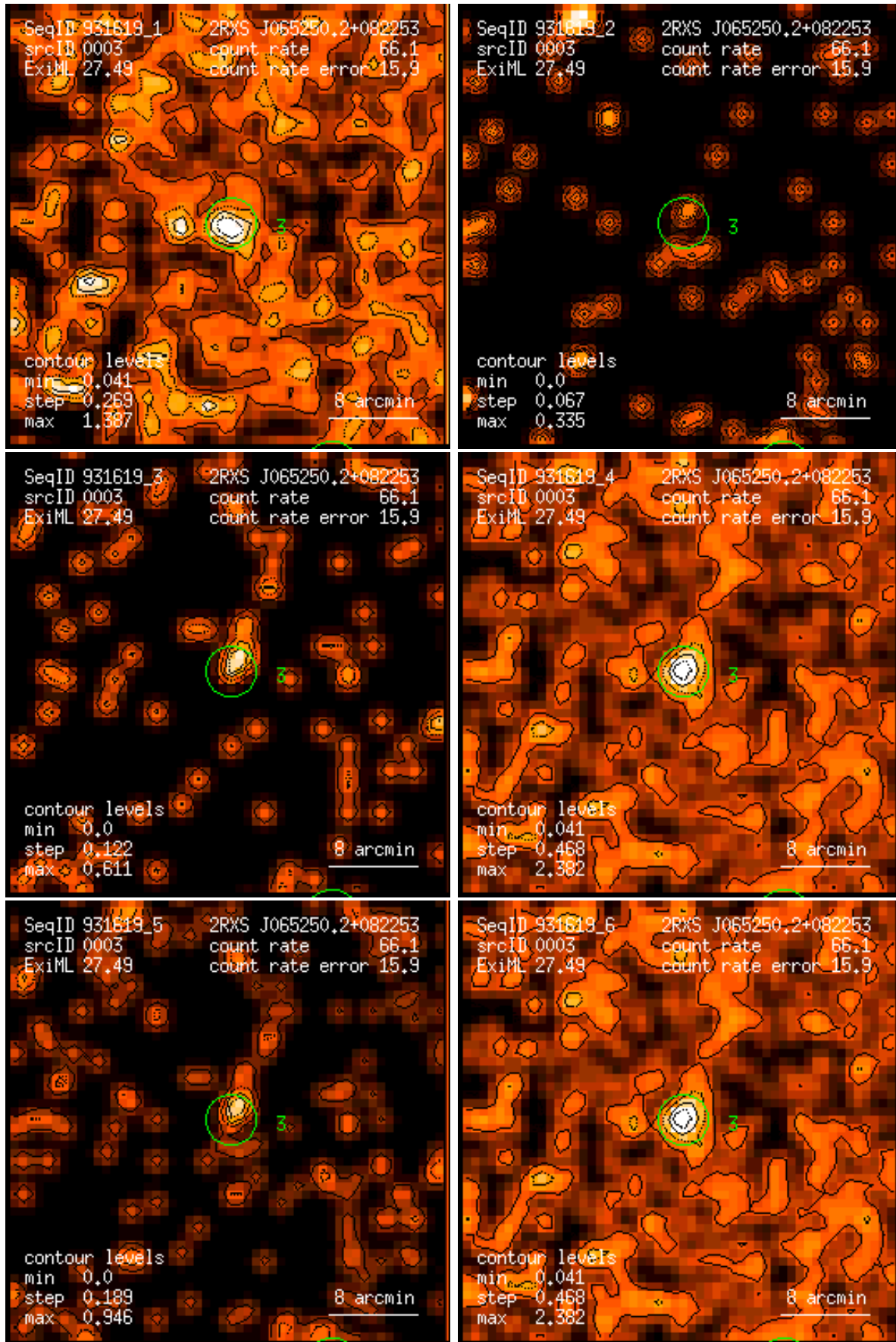
Figure 3: RASS 931619: detection 0003: band rate images, Gaussian filter: (1) PSPC channels 11 – 41, (2) 52 – 90, (3) 91 – 201, (4) 11 – 235, (5) 52 – 201, (6) 11 – 201. Broad band rates in counts/ks. Band rate contour levels in counts/ks/arcmin 2 .
