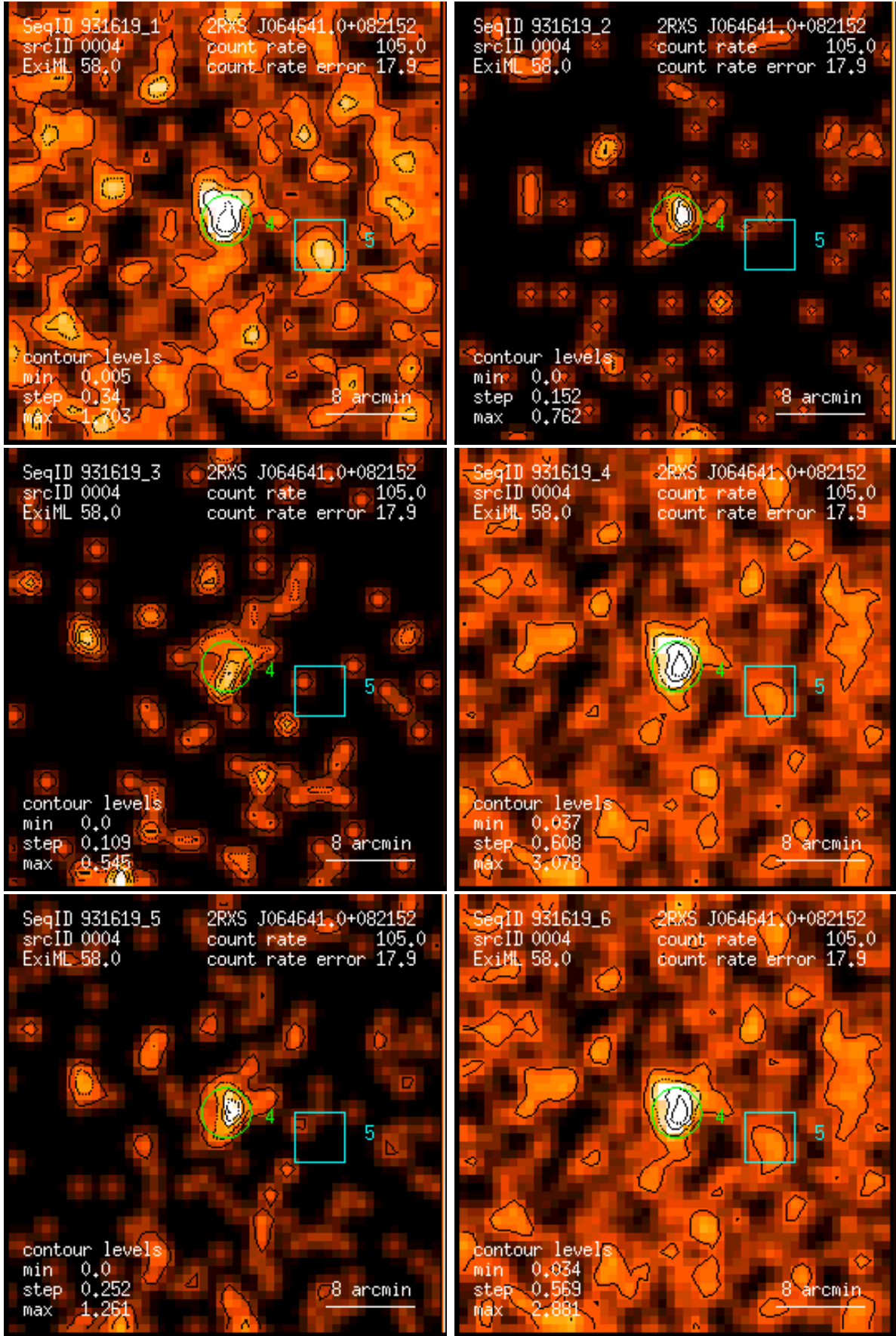
Figure 4: RASS 931619: detection 0004: band rate images, Gaussian filter: (1) PSPC channels 11 – 41, (2) 52 – 90, (3) 91 – 201, (4) 11 – 235, (5) 52 – 201, (6) 11 – 201. Broad band rates in counts/ks. Band rate contour levels in counts/ks/arcmin 2 .
