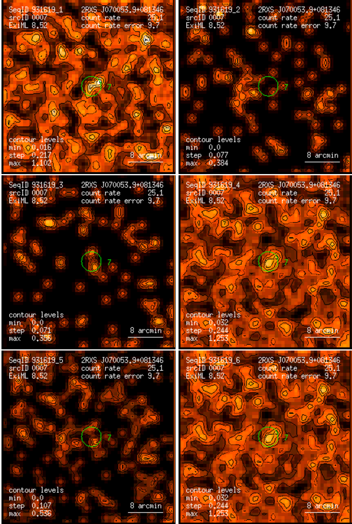
Figure 7: RASS 931619: detection 0007: band rate images, Gaussian filter: (1) PSPC channels 11 – 41, (2) 52 – 90, (3) 91 – 201, (4) 11 – 235, (5) 52 – 201, (6) 11 – 201. Broad band rates in counts/ks. Band rate contour levels in counts/ks/arcmin 2 .
