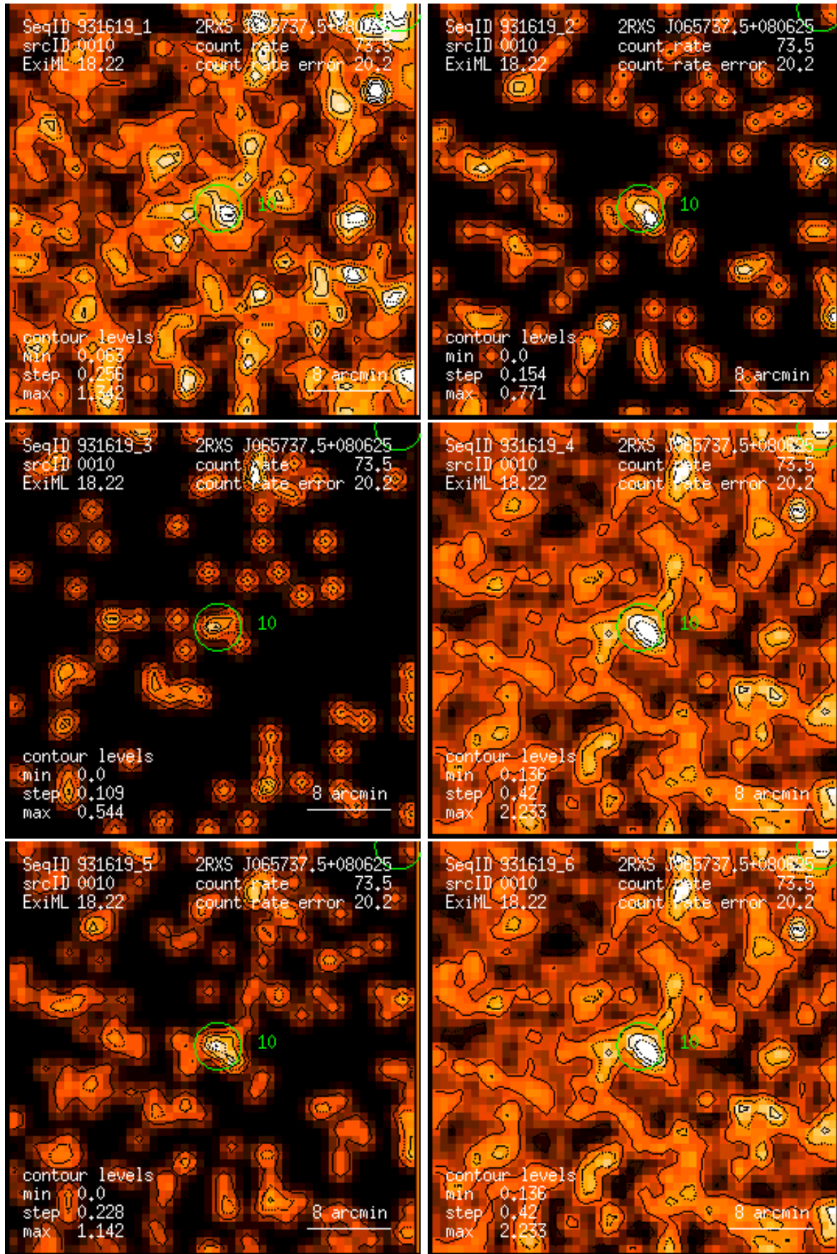
Figure 10: RASS 931619: detection 0010: band rate images, Gaussian filter: (1) PSPC channels 11 – 41, (2) 52 – 90, (3) 91 – 201, (4) 11 – 235, (5) 52 – 201, (6) 11 – 201. Broad band rates in counts/ks. Band rate contour levels in counts/ks/arcmin 2 .
