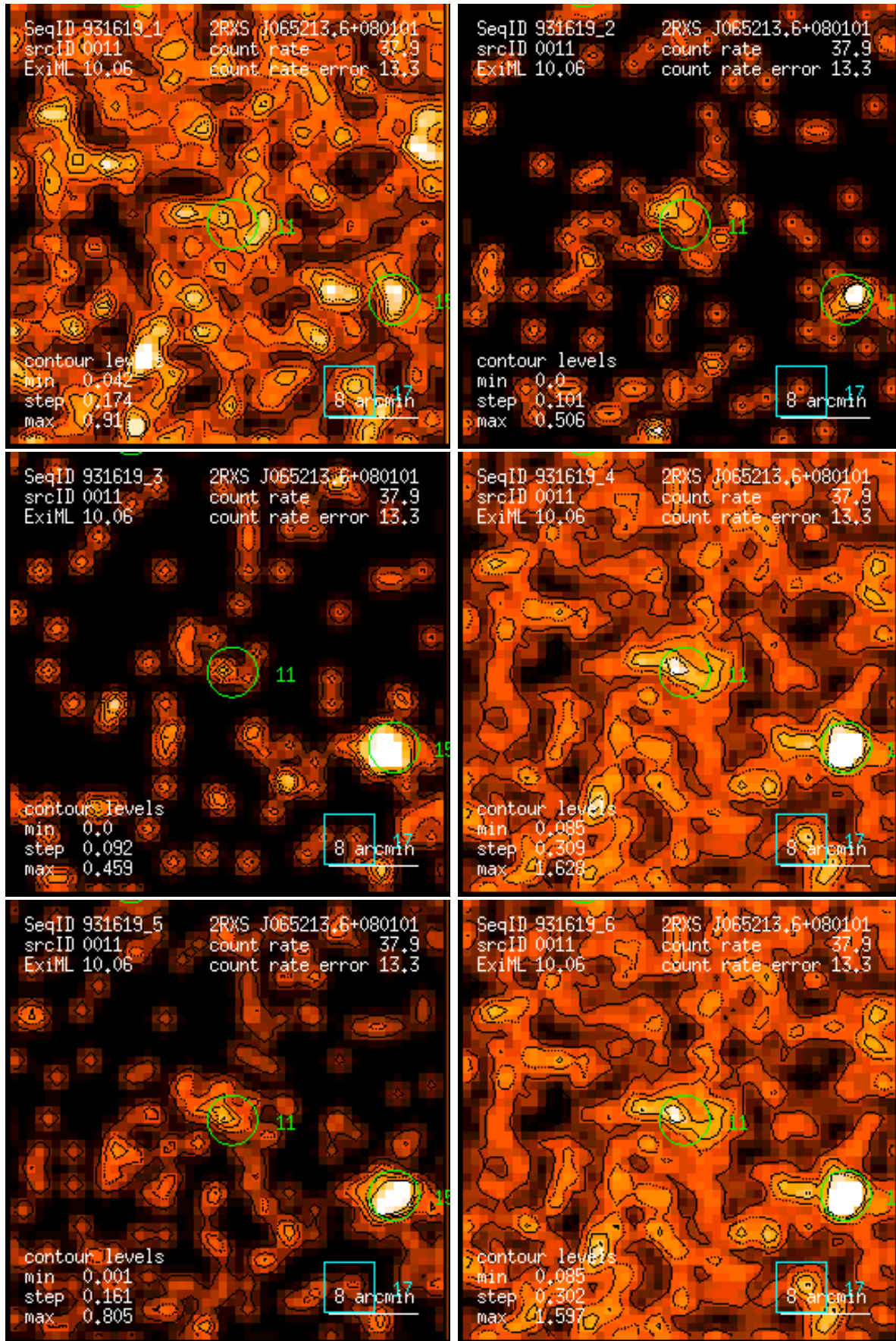
Figure 11: RASS 931619: detection 0011: band rate images, Gaussian filter: (1) PSPC channels 11 – 41, (2) 52 – 90, (3) 91 – 201, (4) 11 – 235, (5) 52 – 201, (6) 11 – 201. Broad band rates in counts/ks. Band rate contour levels in counts/ks/arcmin 2 .
