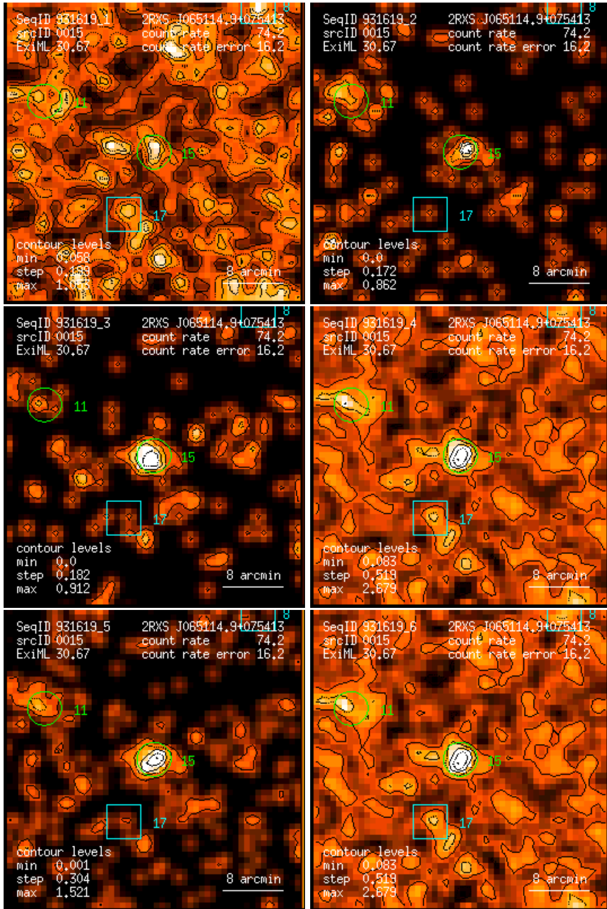
Figure 15: RASS 931619: detection 0015: band rate images, Gaussian filter: (1) PSPC channels 11 – 41, (2) 52 – 90, (3) 91 – 201, (4) 11 – 235, (5) 52 – 201, (6) 11 – 201. Broad band rates in counts/ks. Band rate contour levels in counts/ks/arcmin 2 .
