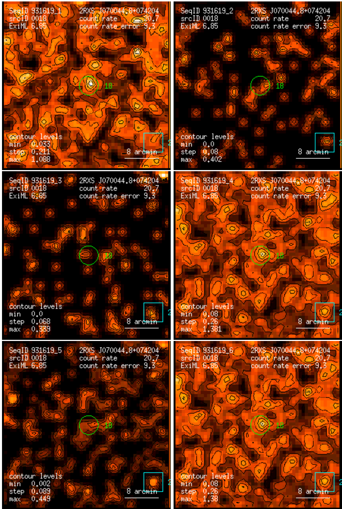
Figure 18: RASS 931619: detection 0018: band rate images, Gaussian filter: (1) PSPC channels 11 – 41, (2) 52 – 90, (3) 91 – 201, (4) 11 – 235, (5) 52 – 201, (6) 11 – 201. Broad band rates in counts/ks. Band rate contour levels in counts/ks/arcmin 2 .
