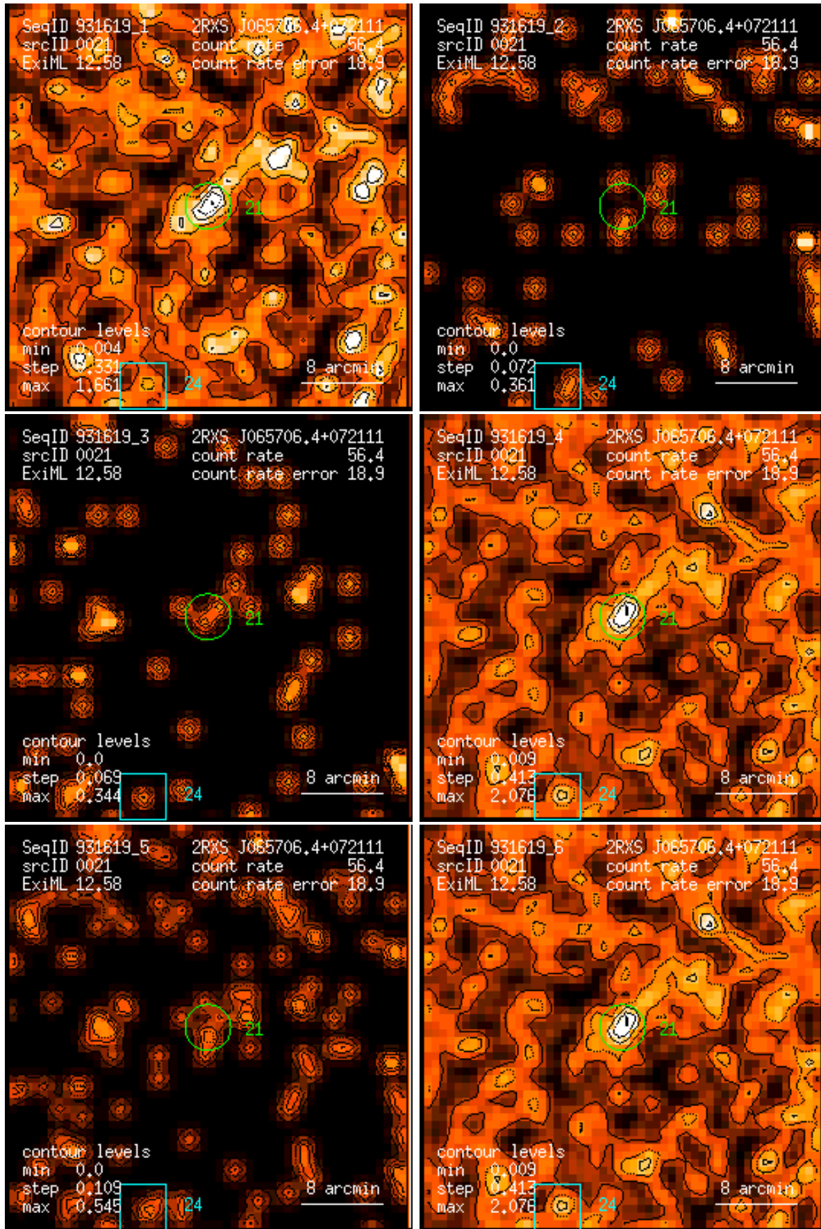
Figure 21: RASS 931619: detection 0021: band rate images, Gaussian filter: (1) PSPC channels 11 – 41, (2) 52 – 90, (3) 91 – 201, (4) 11 – 235, (5) 52 – 201, (6) 11 – 201. Broad band rates in counts/ks. Band rate contour levels in counts/ks/arcmin 2 .
