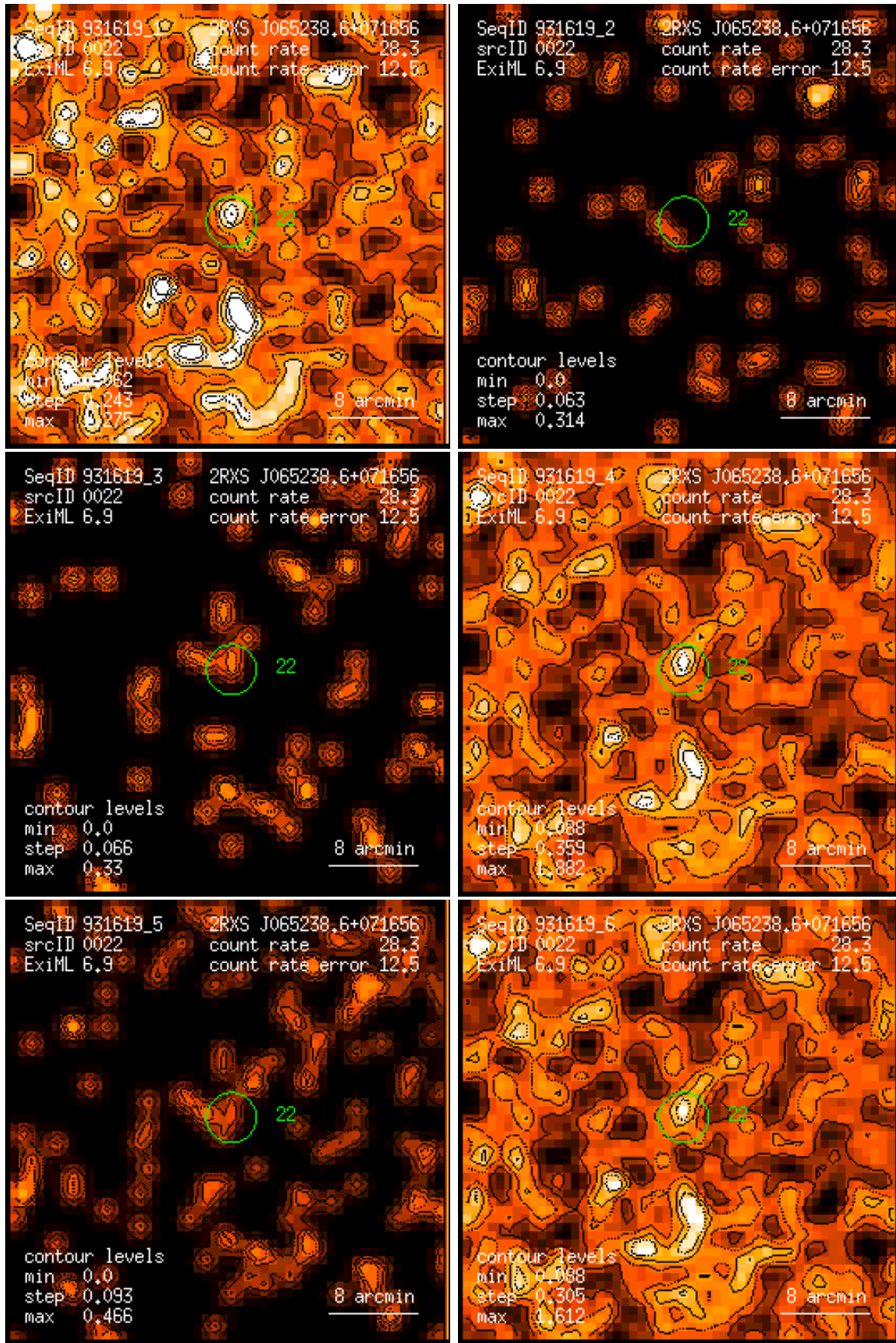
Figure 22: RASS 931619: detection 0022: band rate images, Gaussian filter: (1) PSPC channels 11 – 41, (2) 52 – 90, (3) 91 – 201, (4) 11 – 235, (5) 52 – 201, (6) 11 – 201. Broad band rates in counts/ks. Band rate contour levels in counts/ks/arcmin 2 .
