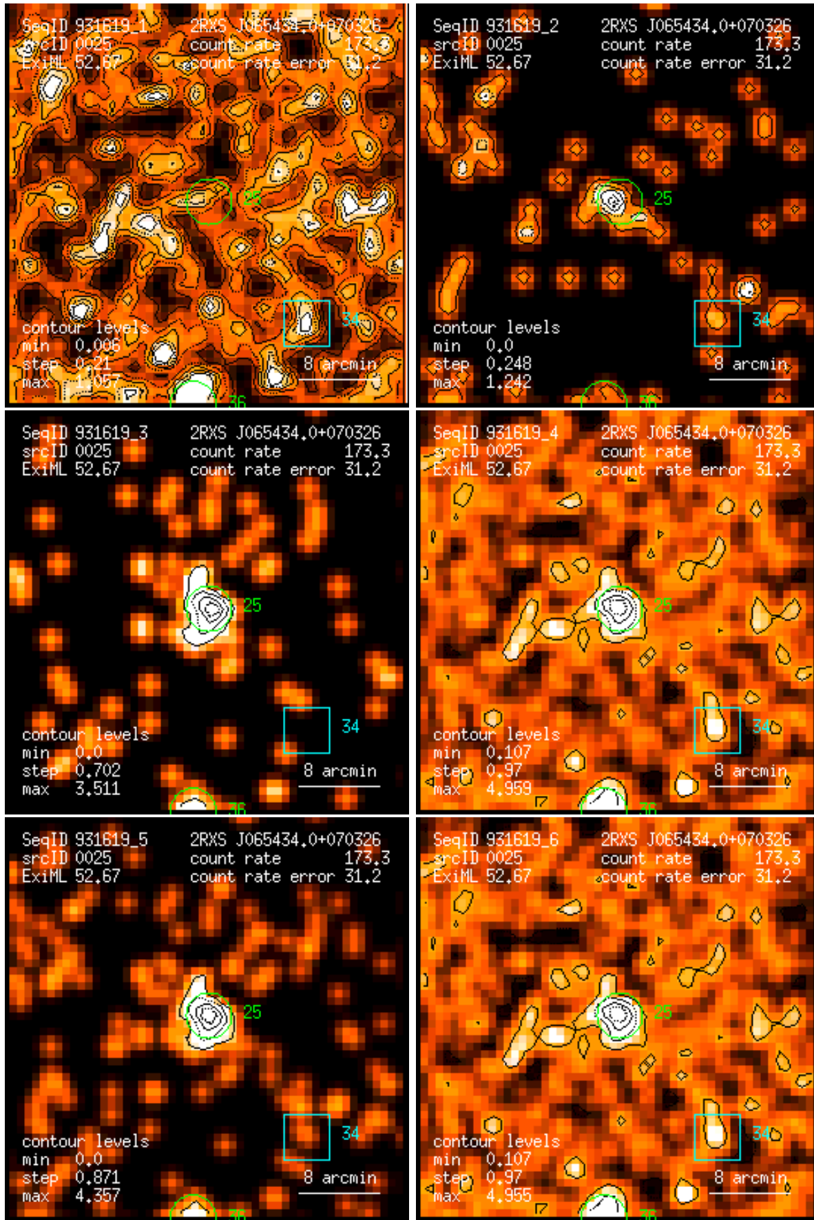
Figure 25: RASS 931619: detection 0025: band rate images, Gaussian filter: (1) PSPC channels 11 – 41, (2) 52 – 90, (3) 91 – 201, (4) 11 – 235, (5) 52 – 201, (6) 11 – 201. Broad band rates in counts/ks. Band rate contour levels in counts/ks/arcmin 2 .
