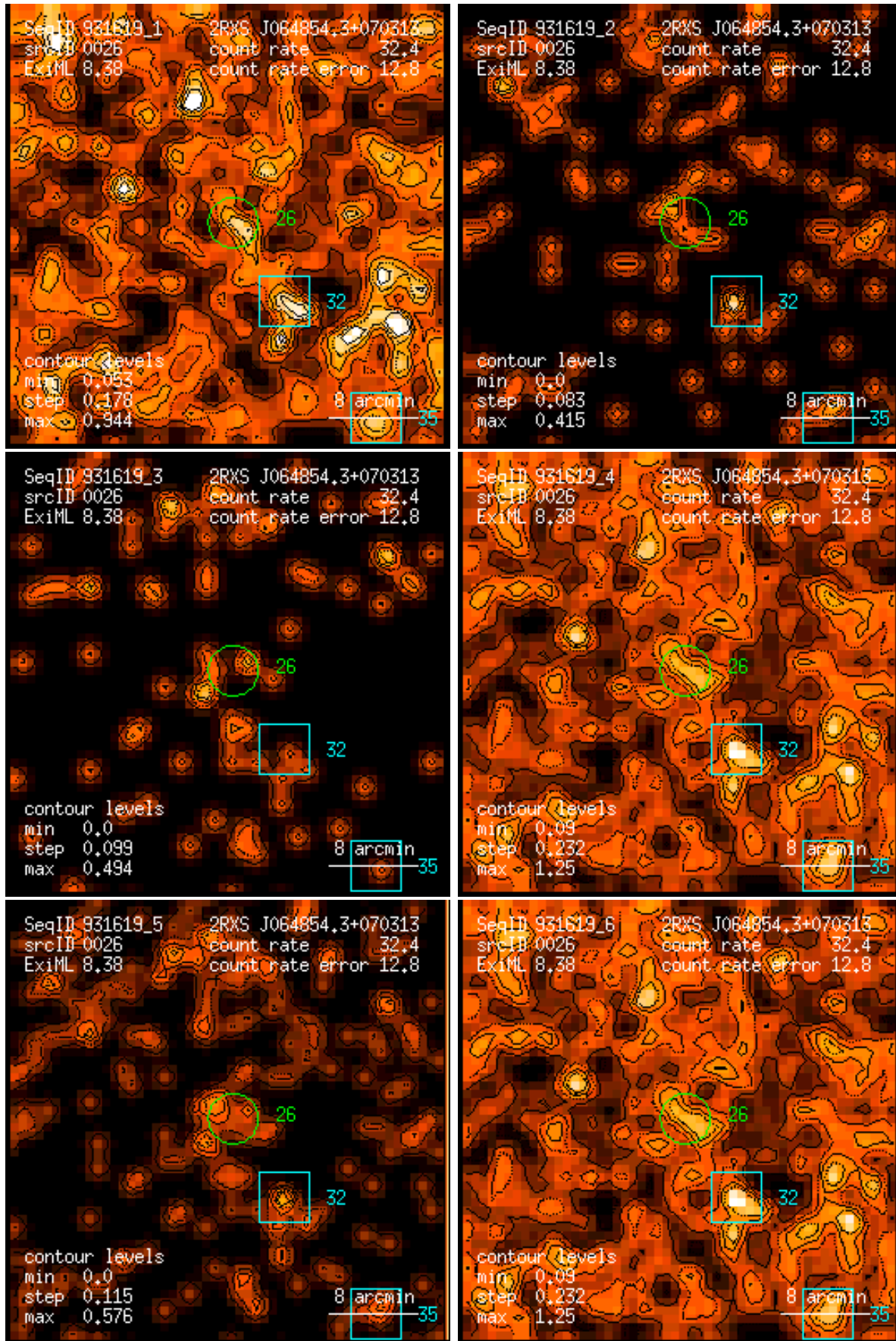
Figure 26: RASS 931619: detection 0026: band rate images, Gaussian filter: (1) PSPC channels 11 – 41, (2) 52 – 90, (3) 91 – 201, (4) 11 – 235, (5) 52 – 201, (6) 11 – 201. Broad band rates in counts/ks. Band rate contour levels in counts/ks/arcmin 2 .
