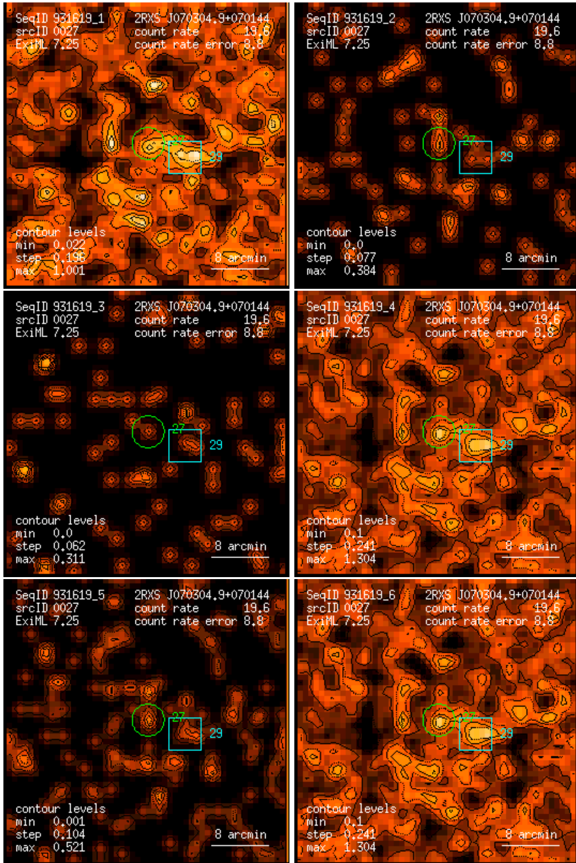
Figure 27: RASS 931619: detection 0027: band rate images, Gaussian filter: (1) PSPC channels 11 – 41, (2) 52 – 90, (3) 91 – 201, (4) 11 – 235, (5) 52 – 201, (6) 11 – 201. Broad band rates in counts/ks. Band rate contour levels in counts/ks/arcmin 2 .
