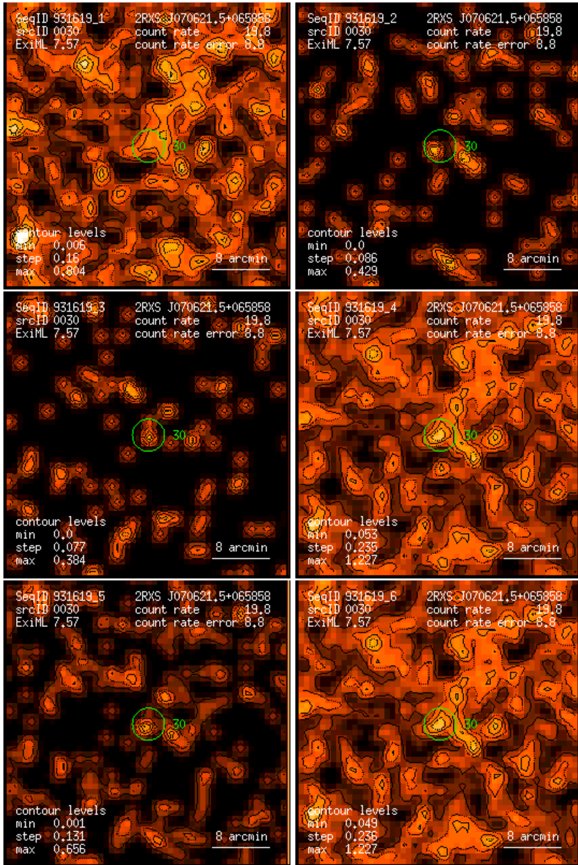
Figure 30: RASS 931619: detection 0030: band rate images, Gaussian filter: (1) PSPC channels 11 – 41, (2) 52 – 90, (3) 91 – 201, (4) 11 – 235, (5) 52 – 201, (6) 11 – 201. Broad band rates in counts/ks. Band rate contour levels in counts/ks/arcmin 2 .
