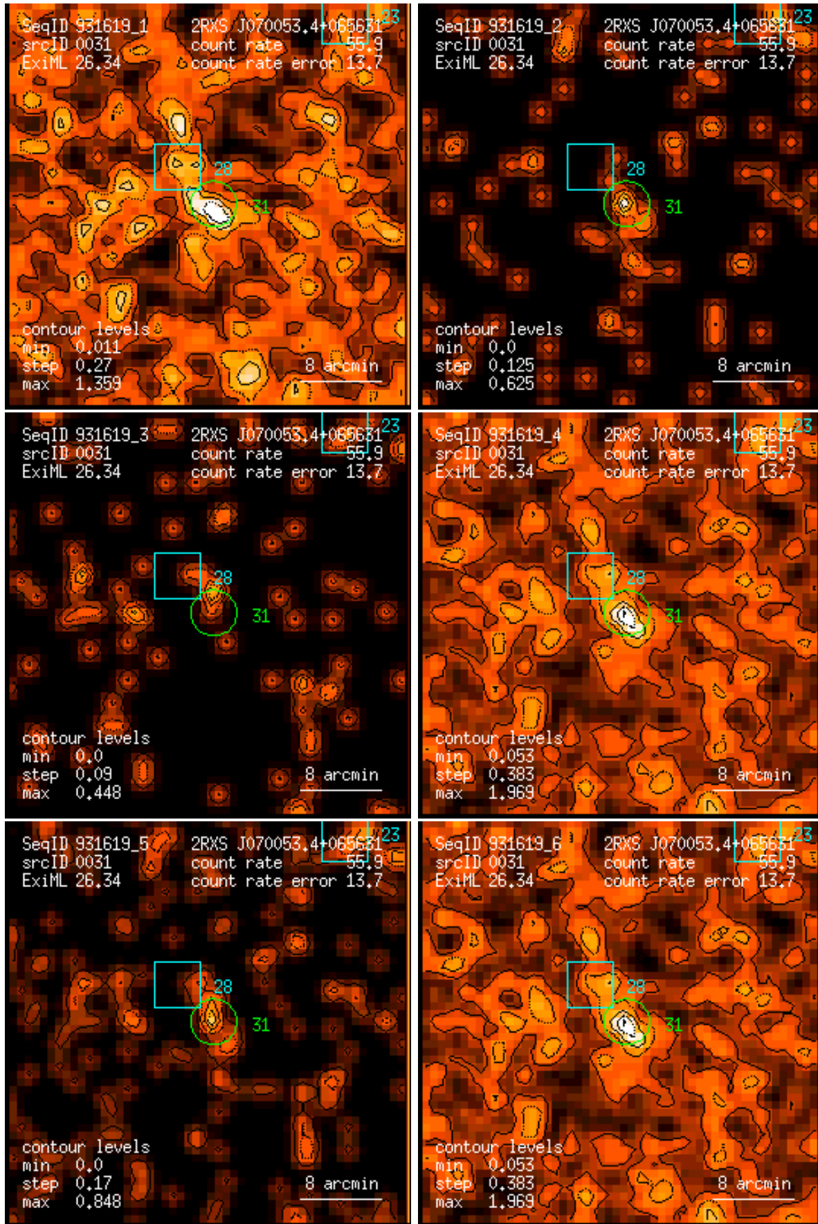
Figure 31: RASS 931619: detection 0031: band rate images, Gaussian filter: (1) PSPC channels 11 – 41, (2) 52 – 90, (3) 91 – 201, (4) 11 – 235, (5) 52 – 201, (6) 11 – 201. Broad band rates in counts/ks. Band rate contour levels in counts/ks/arcmin 2 .
