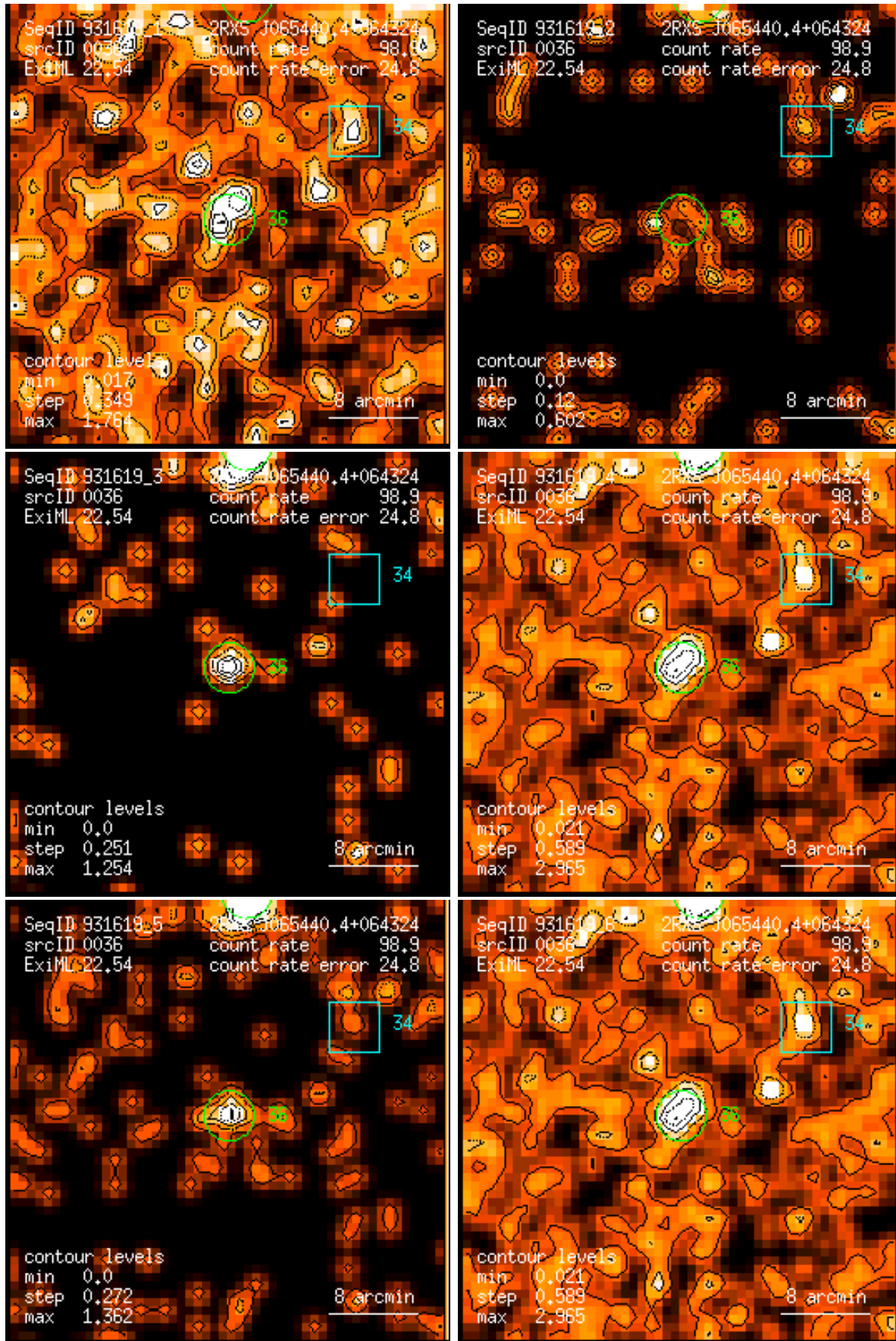
Figure 36: RASS 931619: detection 0036: band rate images, Gaussian filter: (1) PSPC channels 11 – 41, (2) 52 – 90, (3) 91 – 201, (4) 11 – 235, (5) 52 – 201, (6) 11 – 201. Broad band rates in counts/ks. Band rate contour levels in counts/ks/arcmin 2 .
