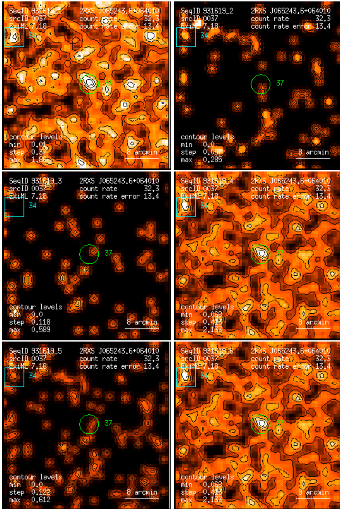
Figure 37: RASS 931619: detection 0037: band rate images, Gaussian filter: (1) PSPC channels 11 – 41, (2) 52 – 90, (3) 91 – 201, (4) 11 – 235, (5) 52 – 201, (6) 11 – 201. Broad band rates in counts/ks. Band rate contour levels in counts/ks/arcmin 2 .
