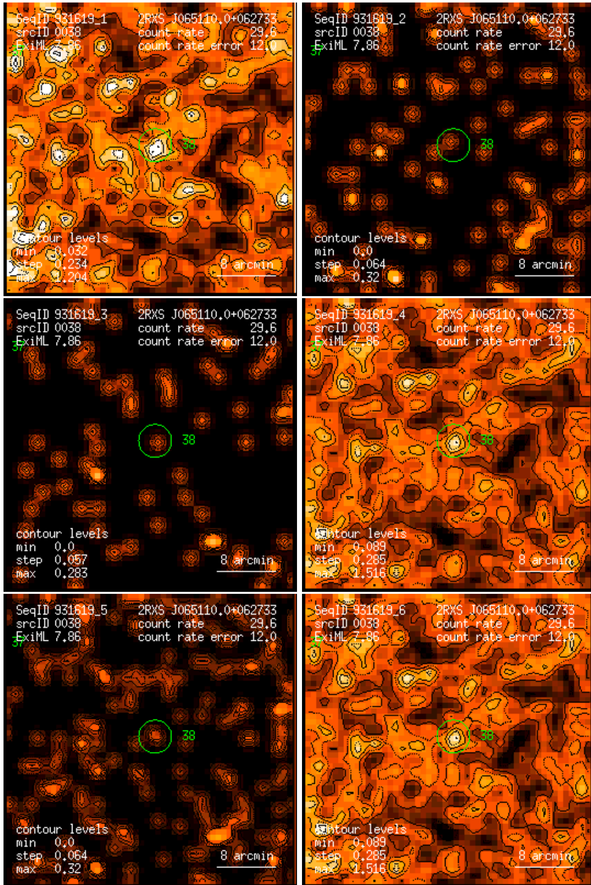
Figure 38: RASS 931619: detection 0038: band rate images, Gaussian filter: (1) PSPC channels 11 – 41, (2) 52 – 90, (3) 91 – 201, (4) 11 – 235, (5) 52 – 201, (6) 11 – 201. Broad band rates in counts/ks. Band rate contour levels in counts/ks/arcmin 2 .
