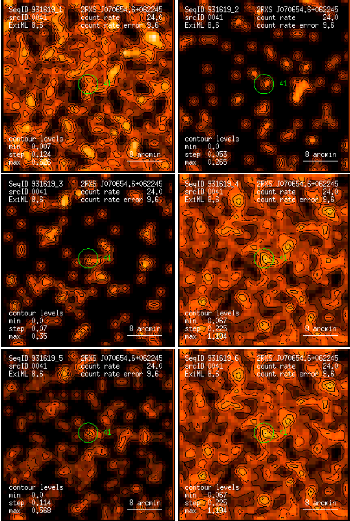
Figure 41: RASS 931619: detection 0041: band rate images, Gaussian filter: (1) PSPC channels 11 – 41, (2) 52 – 90, (3) 91 – 201, (4) 11 – 235, (5) 52 – 201, (6) 11 – 201. Broad band rates in counts/ks. Band rate contour levels in counts/ks/arcmin 2 .
